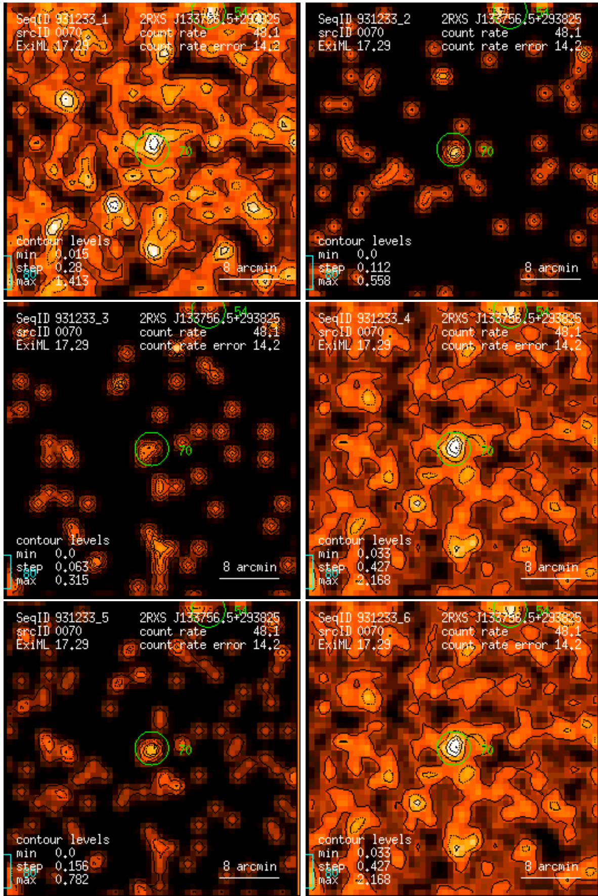
Figure 70: RASS 931233: detection 0070: band rate images, Gaussian filter: (1) PSPC channels 11 – 41, (2) 52 – 90, (3) 91 – 201, (4) 11 – 235, (5) 52 – 201, (6) 11 – 201. Broad band rates in counts/ks. Band rate contour levels in counts/ks/arcmin 2 .
