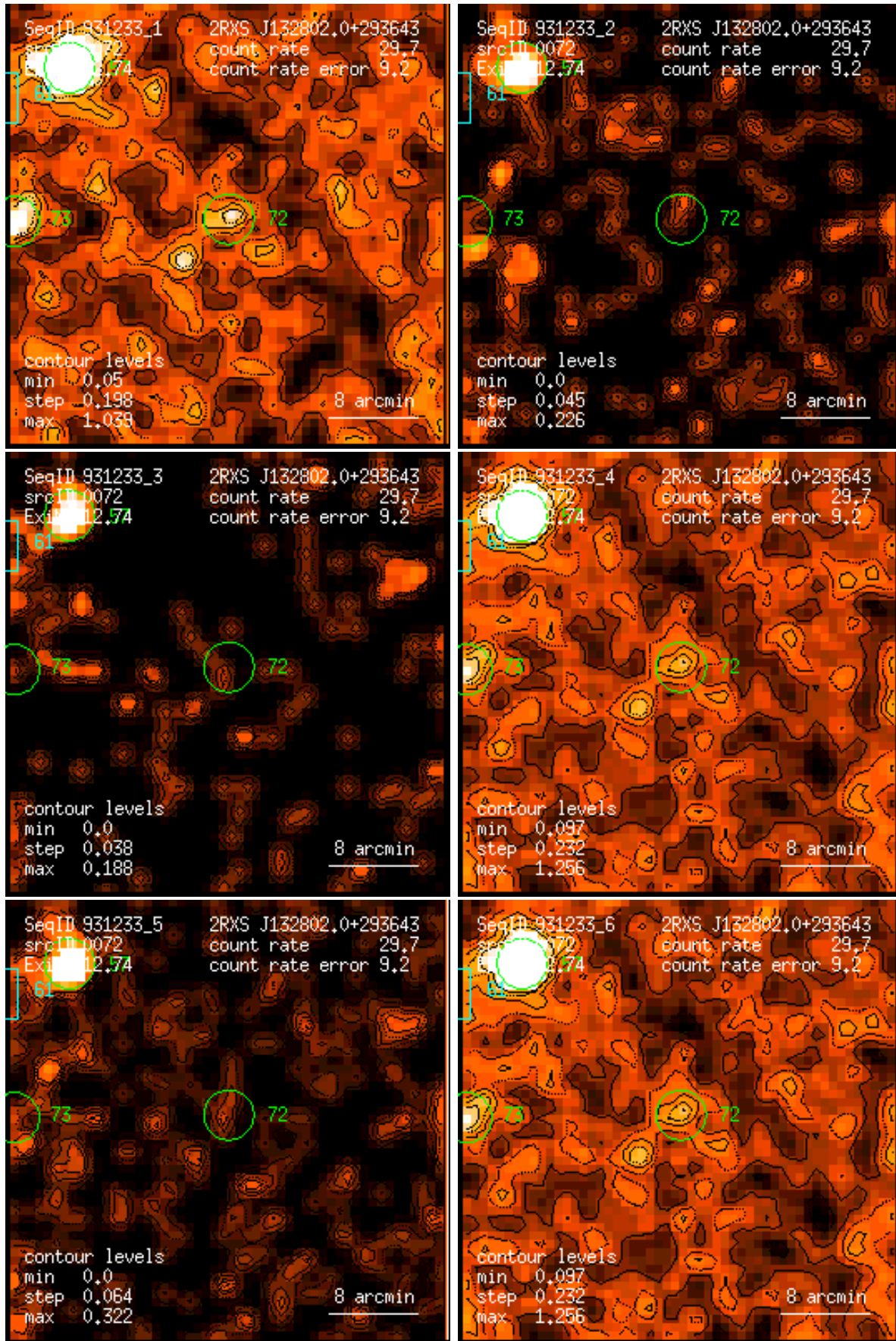
Figure 72: RASS 931233: detection 0072: band rate images, Gaussian filter: (1) PSPC channels 11 – 41, (2) 52 – 90, (3) 91 – 201, (4) 11 – 235, (5) 52 – 201, (6) 11 – 201. Broad band rates in counts/ks. Band rate contour levels in counts/ks/arcmin 2 .
