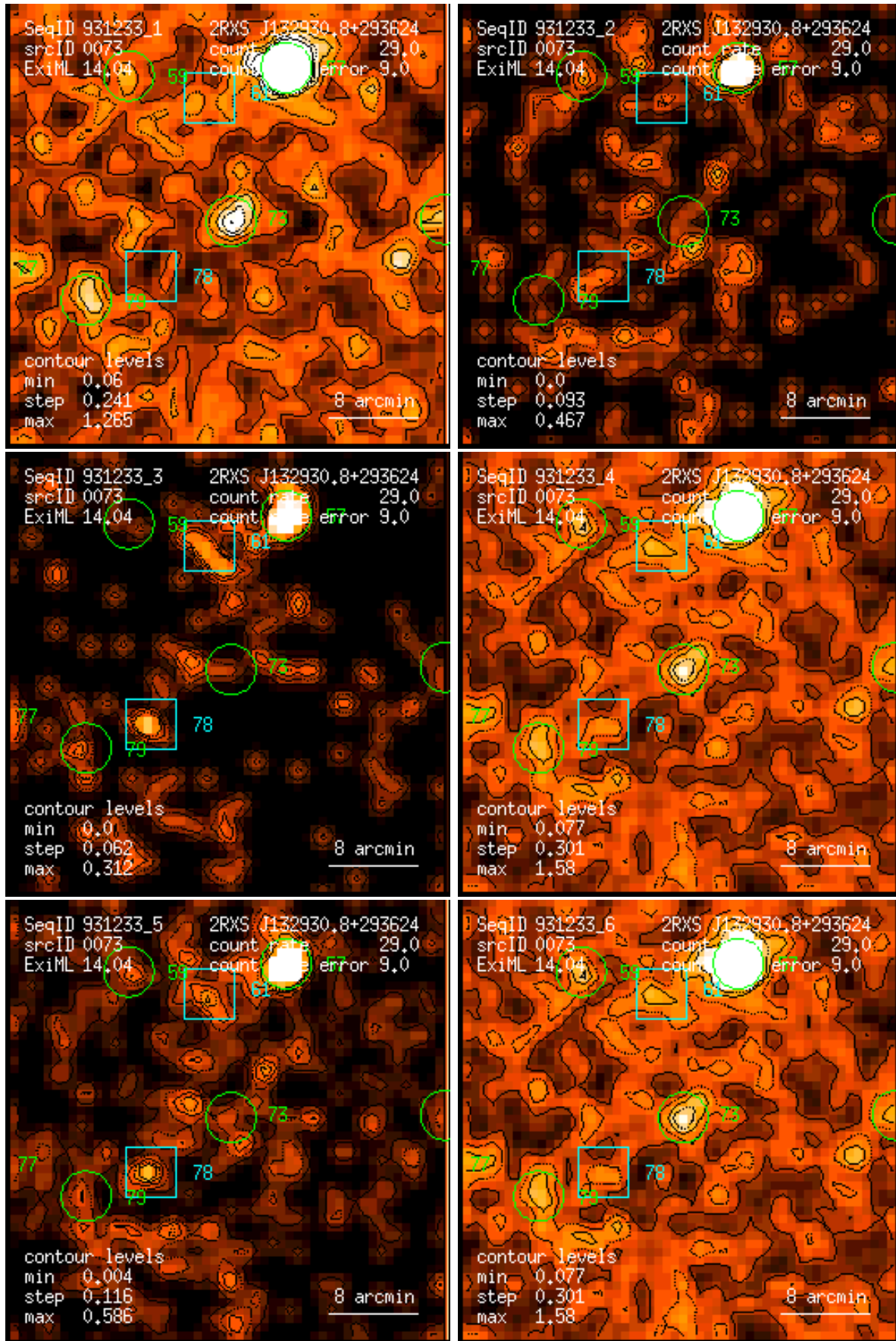
Figure 73: RASS 931233: detection 0073: band rate images, Gaussian filter: (1) PSPC channels 11 – 41, (2) 52 – 90, (3) 91 – 201, (4) 11 – 235, (5) 52 – 201, (6) 11 – 201. Broad band rates in counts/ks. Band rate contour levels in counts/ks/arcmin 2 .
