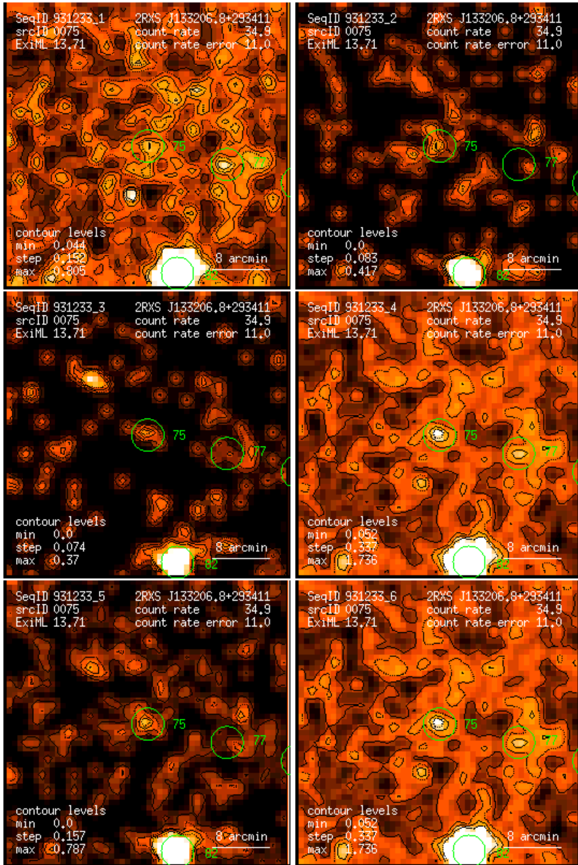
Figure 75: RASS 931233: detection 0075: band rate images, Gaussian filter: (1) PSPC channels 11 – 41, (2) 52 – 90, (3) 91 – 201, (4) 11 – 235, (5) 52 – 201, (6) 11 – 201. Broad band rates in counts/ks. Band rate contour levels in counts/ks/arcmin 2 .
