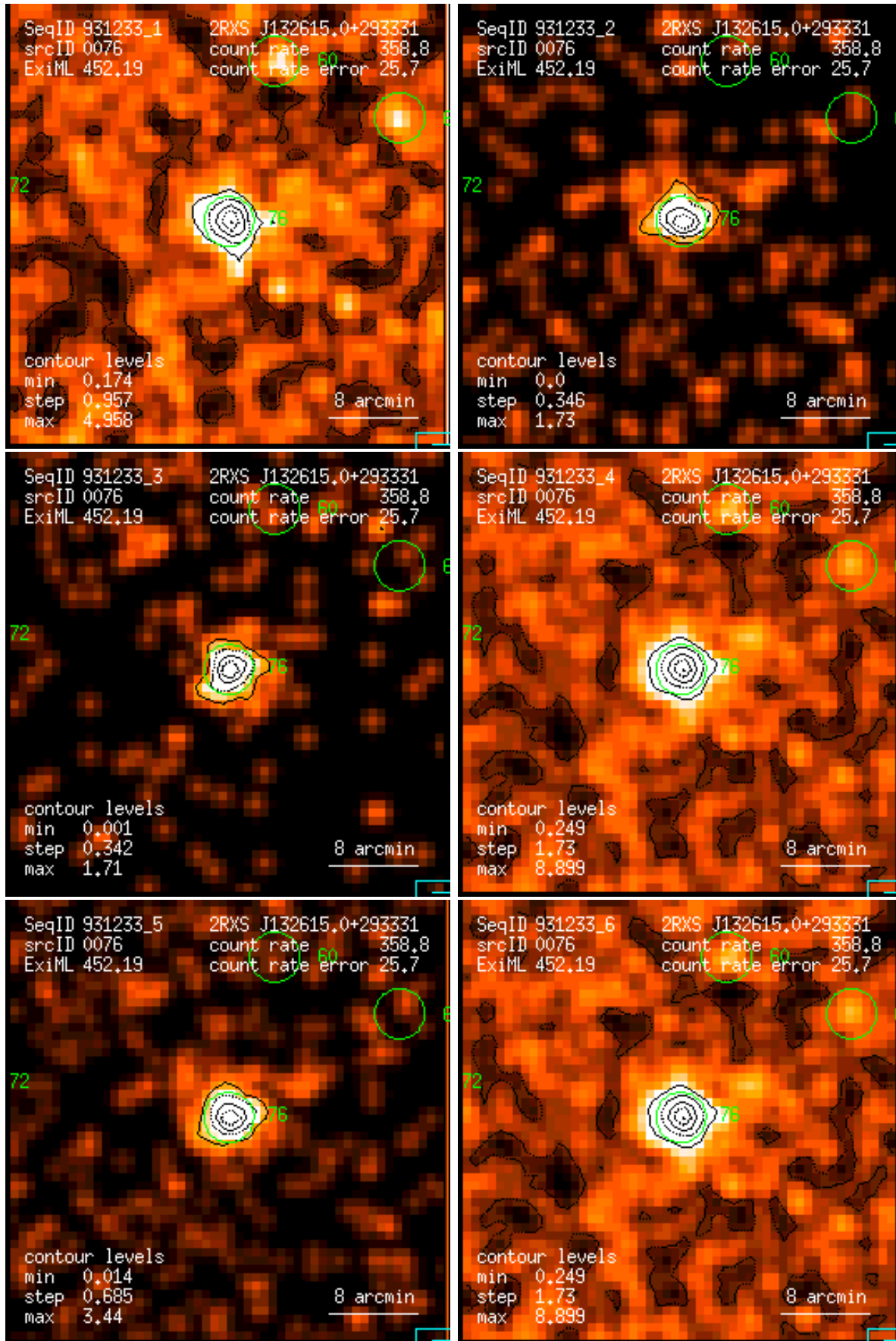
Figure 76: RASS 931233: detection 0076: band rate images, Gaussian filter: (1) PSPC channels 11 – 41, (2) 52 – 90, (3) 91 – 201, (4) 11 – 235, (5) 52 – 201, (6) 11 – 201. Broad band rates in counts/ks. Band rate contour levels in counts/ks/arcmin 2 .
