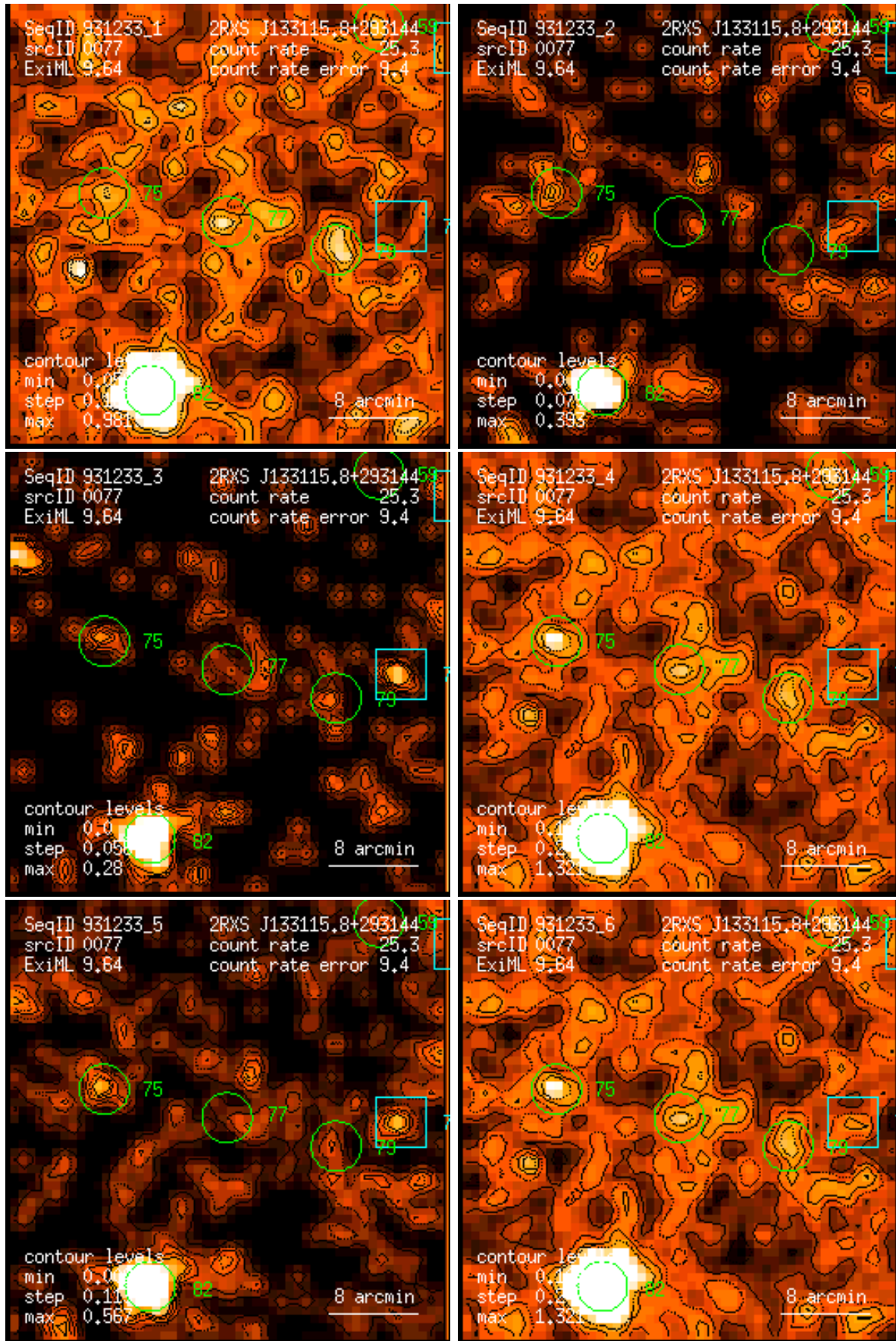
Figure 77: RASS 931233: detection 0077: band rate images, Gaussian filter: (1) PSPC channels 11 – 41, (2) 52 – 90, (3) 91 – 201, (4) 11 – 235, (5) 52 – 201, (6) 11 – 201. Broad band rates in counts/ks. Band rate contour levels in counts/ks/arcmin 2 .
