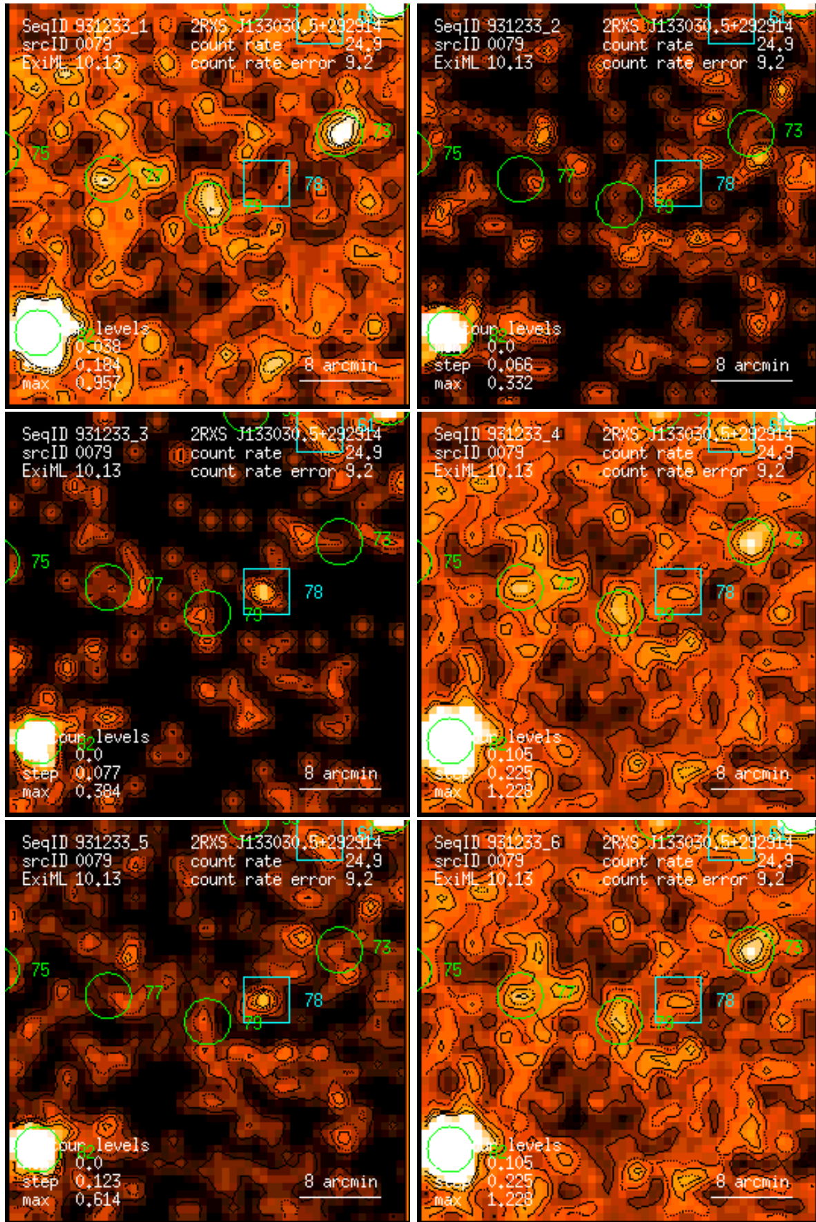
Figure 79: RASS 931233: detection 0079: band rate images, Gaussian filter: (1) PSPC channels 11 – 41, (2) 52 – 90, (3) 91 – 201, (4) 11 – 235, (5) 52 – 201, (6) 11 – 201. Broad band rates in counts/ks. Band rate contour levels in counts/ks/arcmin 2 .
