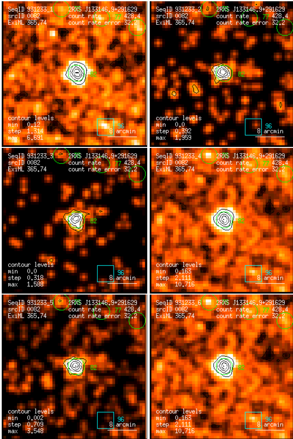
Figure 82: RASS 931233: detection 0082: band rate images, Gaussian filter: (1) PSPC channels 11 – 41, (2) 52 – 90, (3) 91 – 201, (4) 11 – 235, (5) 52 – 201, (6) 11 – 201. Broad band rates in counts/ks. Band rate contour levels in counts/ks/arcmin 2 .
