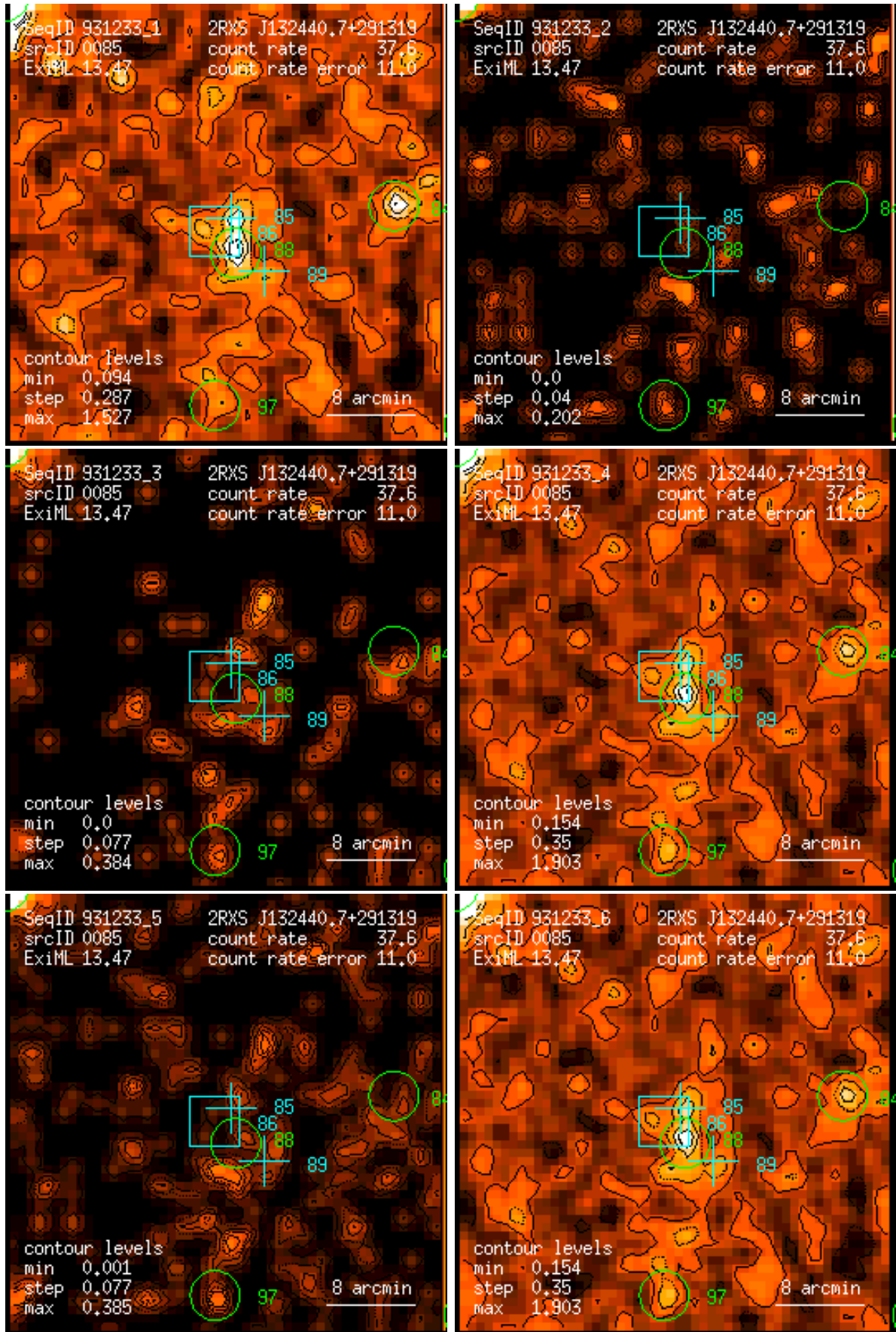
Figure 85: RASS 931233: detection 0085: band rate images, Gaussian filter: (1) PSPC channels 11 – 41, (2) 52 – 90, (3) 91 – 201, (4) 11 – 235, (5) 52 – 201, (6) 11 – 201. Broad band rates in counts/ks. Band rate contour levels in counts/ks/arcmin 2 .
