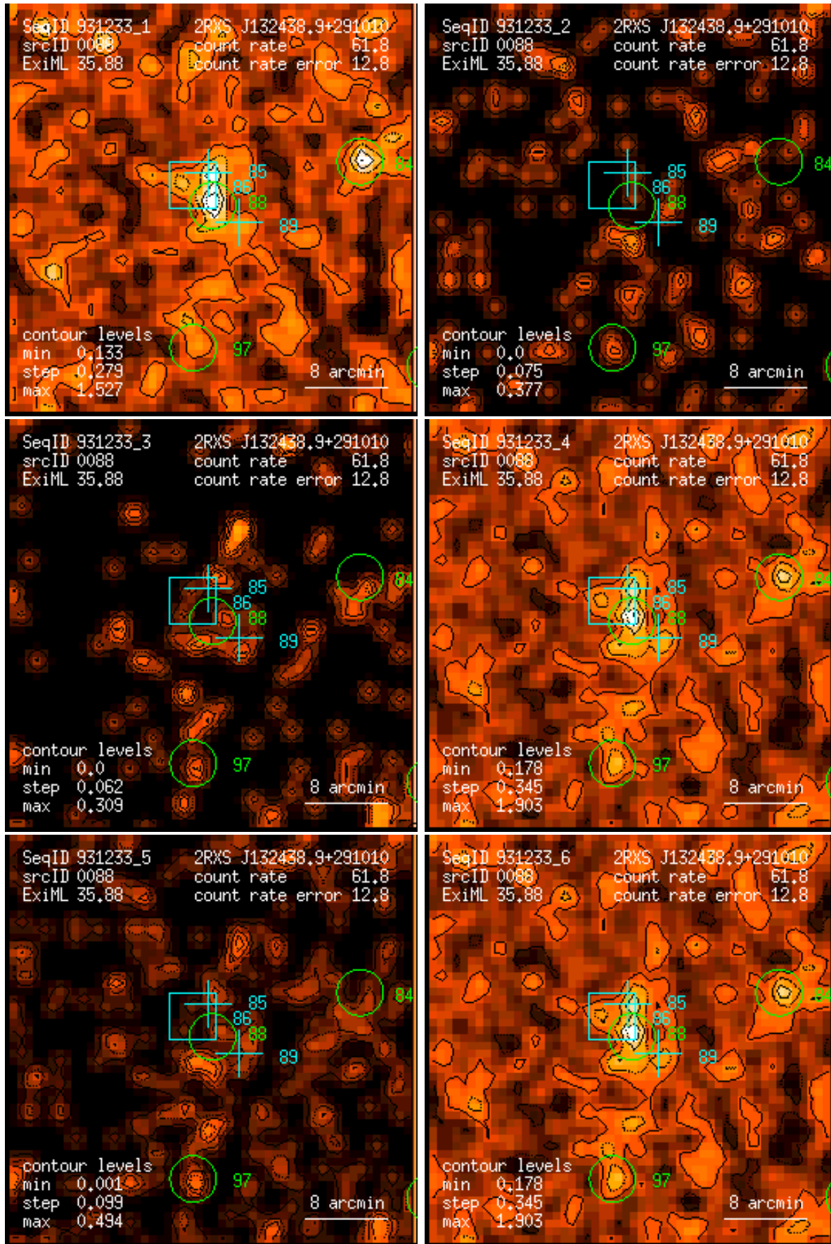
Figure 88: RASS 931233: detection 0088: band rate images, Gaussian filter: (1) PSPC channels 11 – 41, (2) 52 – 90, (3) 91 – 201, (4) 11 – 235, (5) 52 – 201, (6) 11 – 201. Broad band rates in counts/ks. Band rate contour levels in counts/ks/arcmin 2 .
