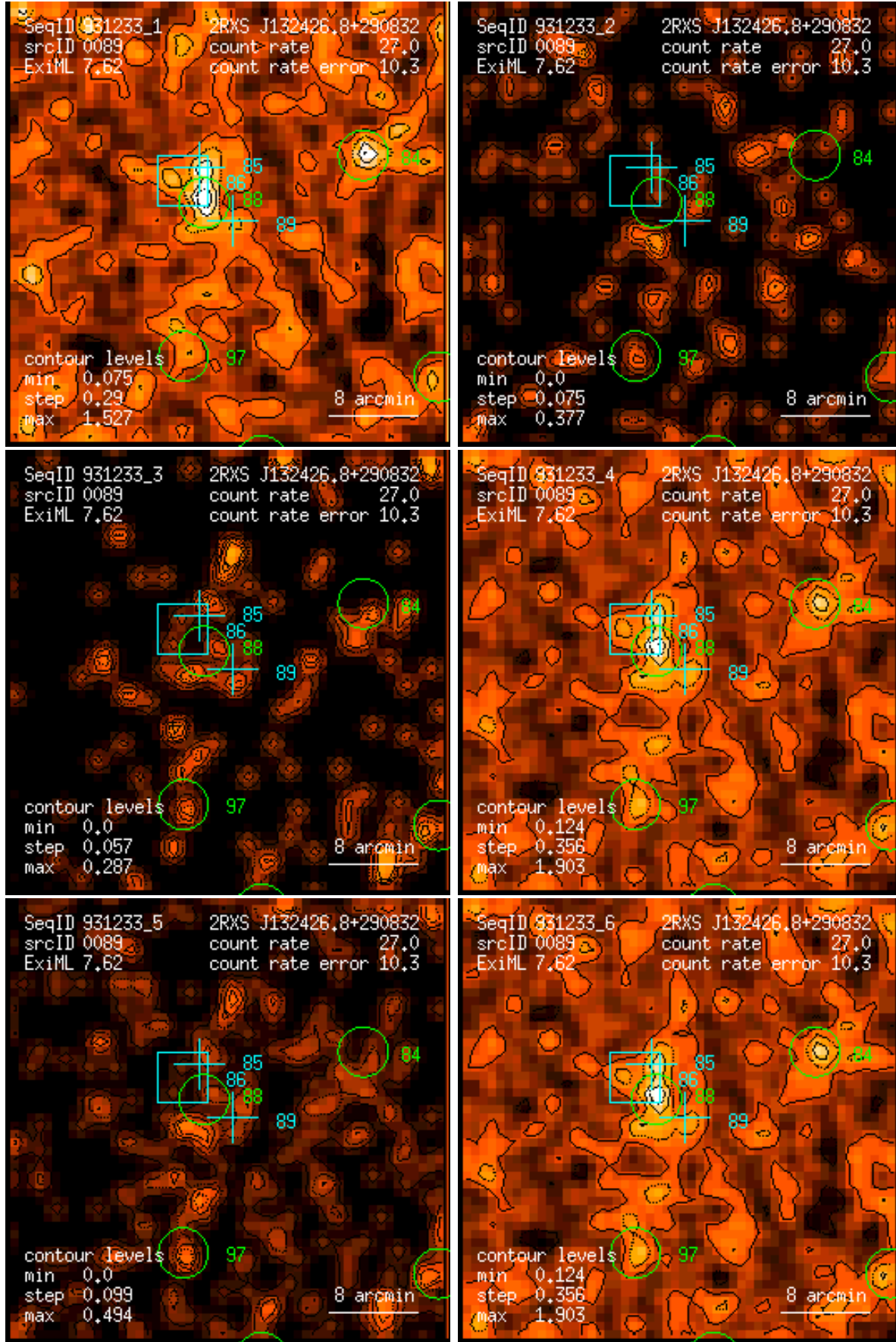
Figure 89: RASS 931233: detection 0089: band rate images, Gaussian filter: (1) PSPC channels 11 – 41, (2) 52 – 90, (3) 91 – 201, (4) 11 – 235, (5) 52 – 201, (6) 11 – 201. Broad band rates in counts/ks. Band rate contour levels in counts/ks/arcmin 2 .
