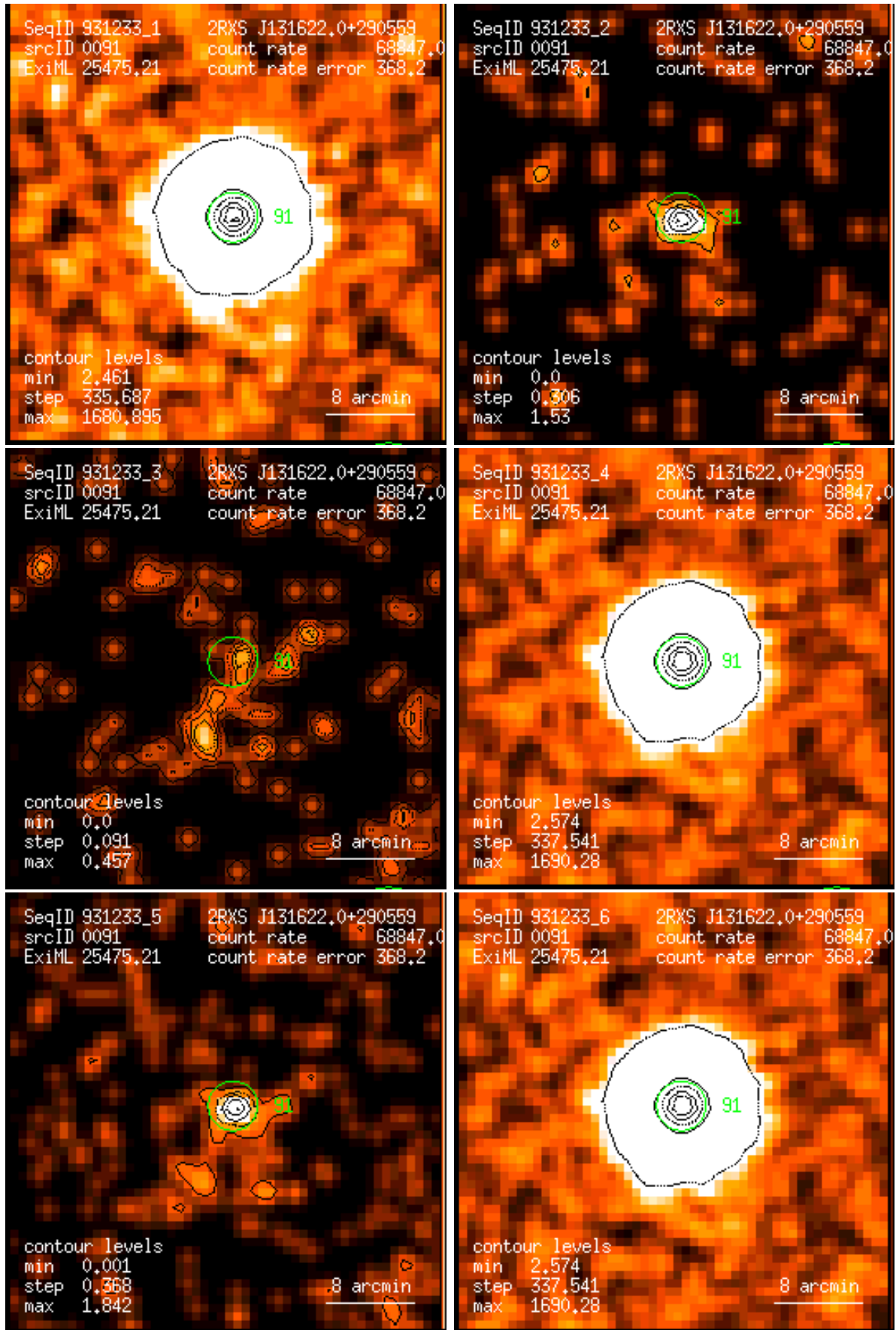
Figure 91: RASS 931233: detection 0091: band rate images, Gaussian filter: (1) PSPC channels 11 – 41, (2) 52 – 90, (3) 91 – 201, (4) 11 – 235, (5) 52 – 201, (6) 11 – 201. Broad band rates in counts/ks. Band rate contour levels in counts/ks/arcmin 2 .
