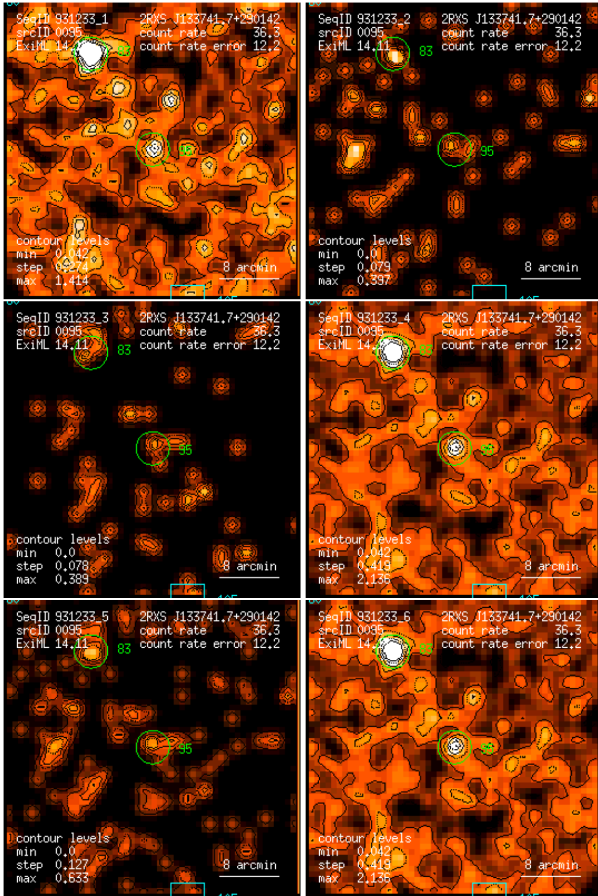
Figure 95: RASS 931233: detection 0095: band rate images, Gaussian filter: (1) PSPC channels 11 – 41, (2) 52 – 90, (3) 91 – 201, (4) 11 – 235, (5) 52 – 201, (6) 11 – 201. Broad band rates in counts/ks. Band rate contour levels in counts/ks/arcmin 2 .
