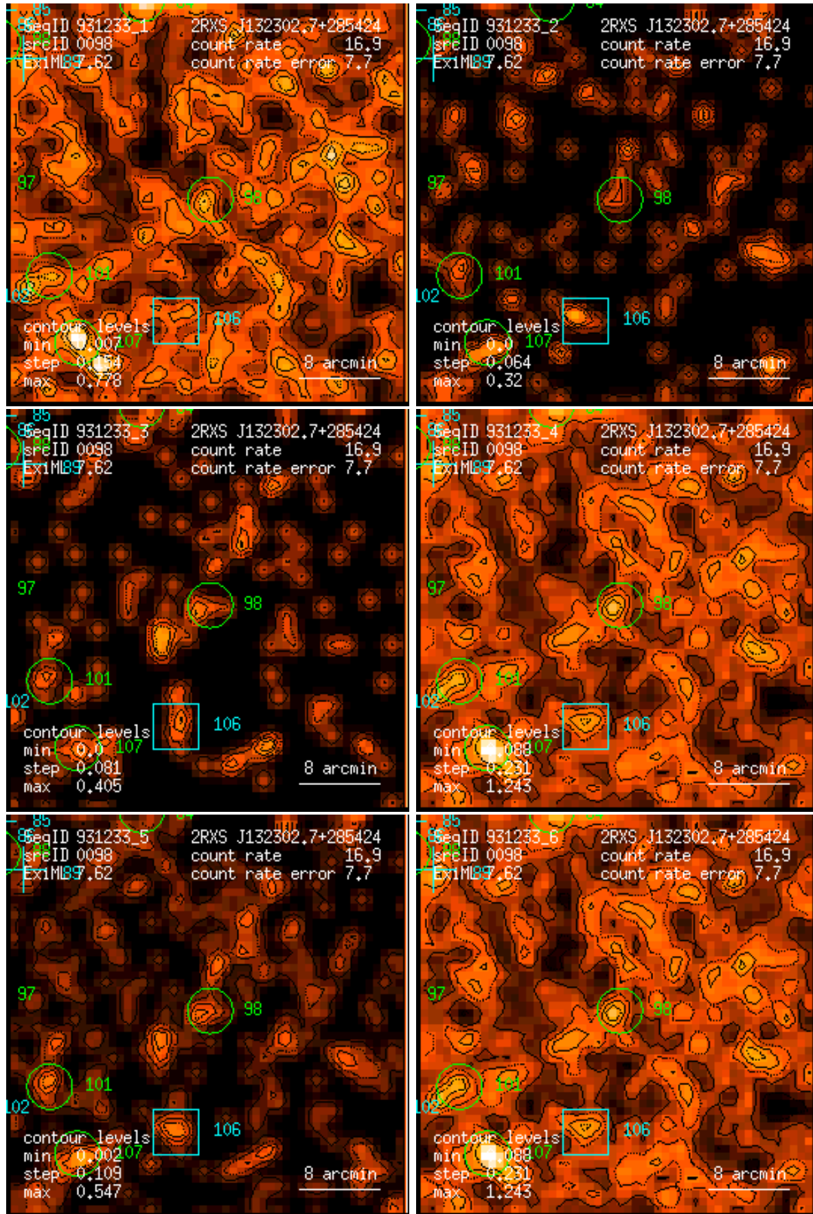
Figure 98: RASS 931233: detection 0098: band rate images, Gaussian filter: (1) PSPC channels 11 – 41, (2) 52 – 90, (3) 91 – 201, (4) 11 – 235, (5) 52 – 201, (6) 11 – 201. Broad band rates in counts/ks. Band rate contour levels in counts/ks/arcmin 2 .
