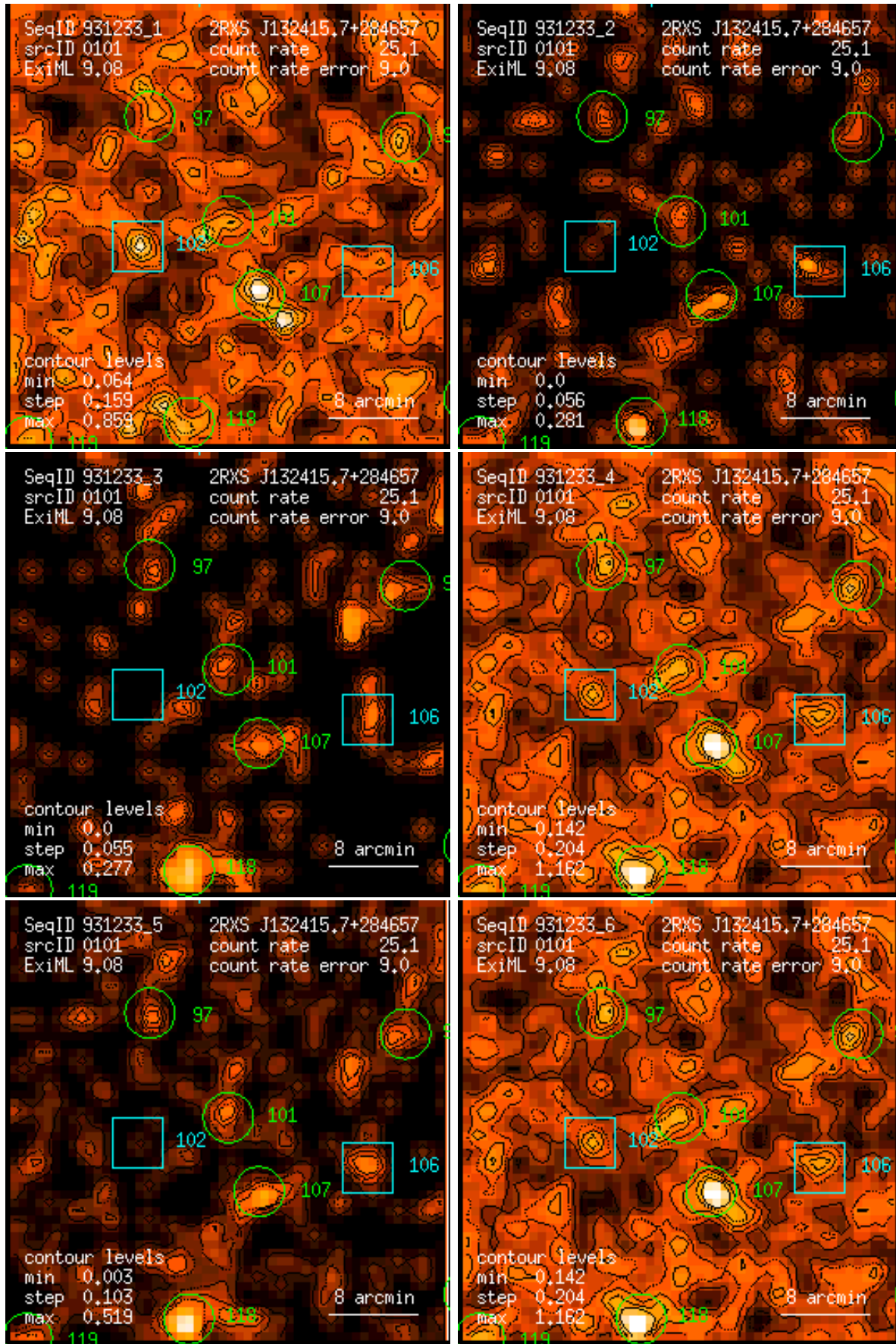
Figure 101: RASS 931233: detection 0101: band rate images, Gaussian filter: (1) PSPC channels 11 – 41, (2) 52 – 90, (3) 91 – 201, (4) 11 – 235, (5) 52 – 201, (6) 11 – 201. Broad band rates in counts/ks. Band rate contour levels in counts/ks/arcmin 2 .
