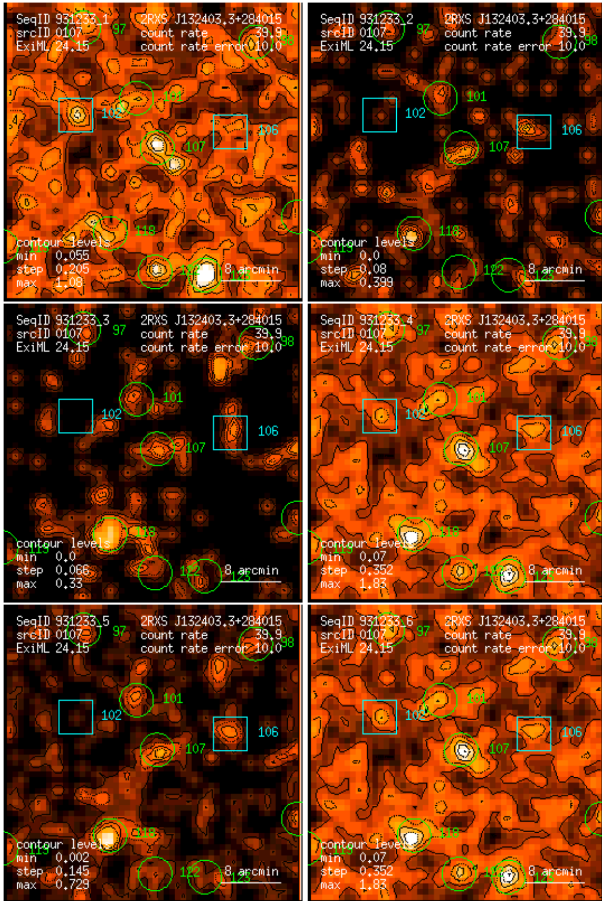
Figure 107: RASS 931233: detection 0107: band rate images, Gaussian filter: (1) PSPC channels 11 – 41, (2) 52 – 90, (3) 91 – 201, (4) 11 – 235, (5) 52 – 201, (6) 11 – 201. Broad band rates in counts/ks. Band rate contour levels in counts/ks/arcmin 2 .
