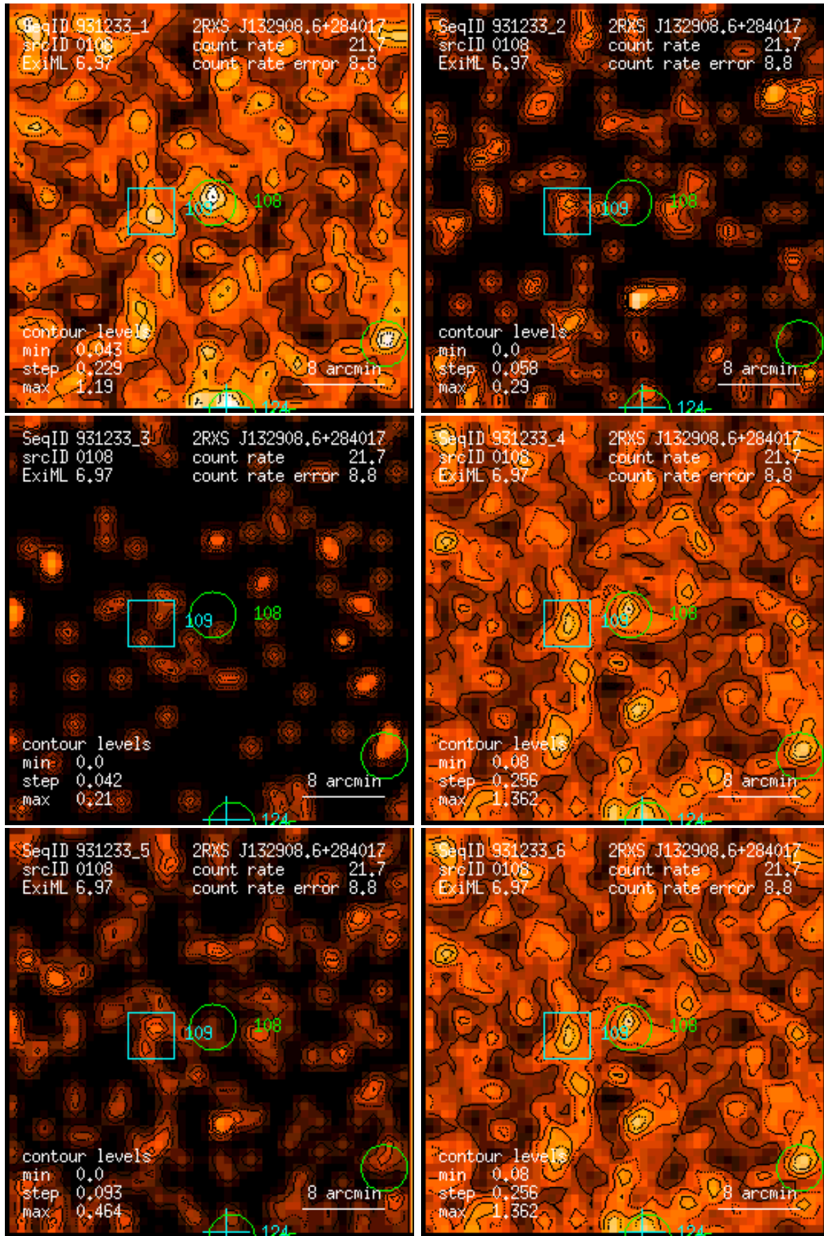
Figure 108: RASS 931233: detection 0108: band rate images, Gaussian filter: (1) PSPC channels 11 – 41, (2) 52 – 90, (3) 91 – 201, (4) 11 – 235, (5) 52 – 201, (6) 11 – 201. Broad band rates in counts/ks. Band rate contour levels in counts/ks/arcmin 2 .
