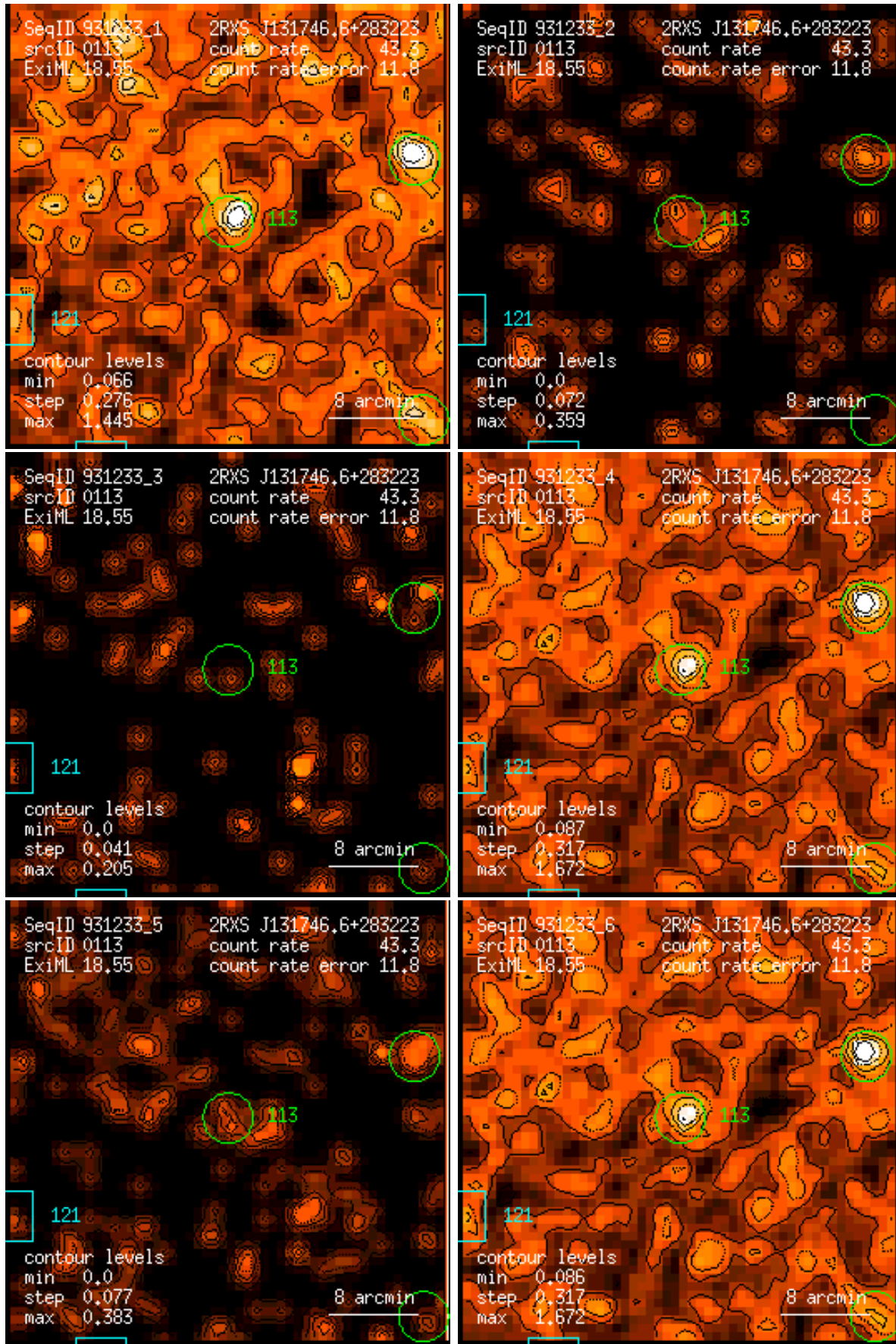
Figure 113: RASS 931233: detection 0113: band rate images, Gaussian filter: (1) PSPC channels 11 – 41, (2) 52 – 90, (3) 91 – 201, (4) 11 – 235, (5) 52 – 201, (6) 11 – 201. Broad band rates in counts/ks. Band rate contour levels in counts/ks/arcmin 2 .
