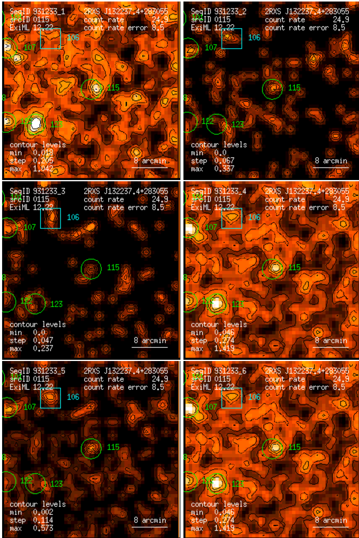
Figure 115: RASS 931233: detection 0115: band rate images, Gaussian filter: (1) PSPC channels 11 – 41, (2) 52 – 90, (3) 91 – 201, (4) 11 – 235, (5) 52 – 201, (6) 11 – 201. Broad band rates in counts/ks. Band rate contour levels in counts/ks/arcmin 2 .
