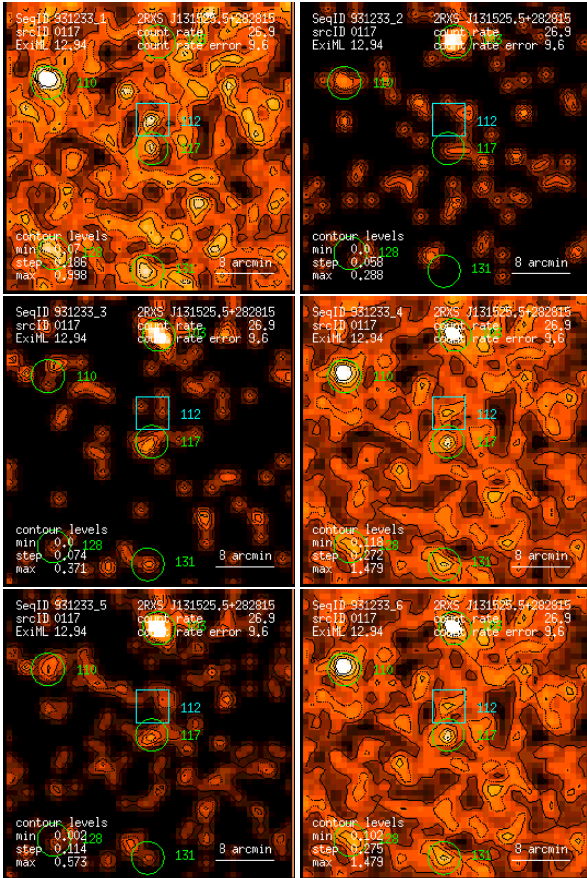
Figure 117: RASS 931233: detection 0117: band rate images, Gaussian filter: (1) PSPC channels 11 – 41, (2) 52 – 90, (3) 91 – 201, (4) 11 – 235, (5) 52 – 201, (6) 11 – 201. Broad band rates in counts/ks. Band rate contour levels in counts/ks/arcmin 2 .
