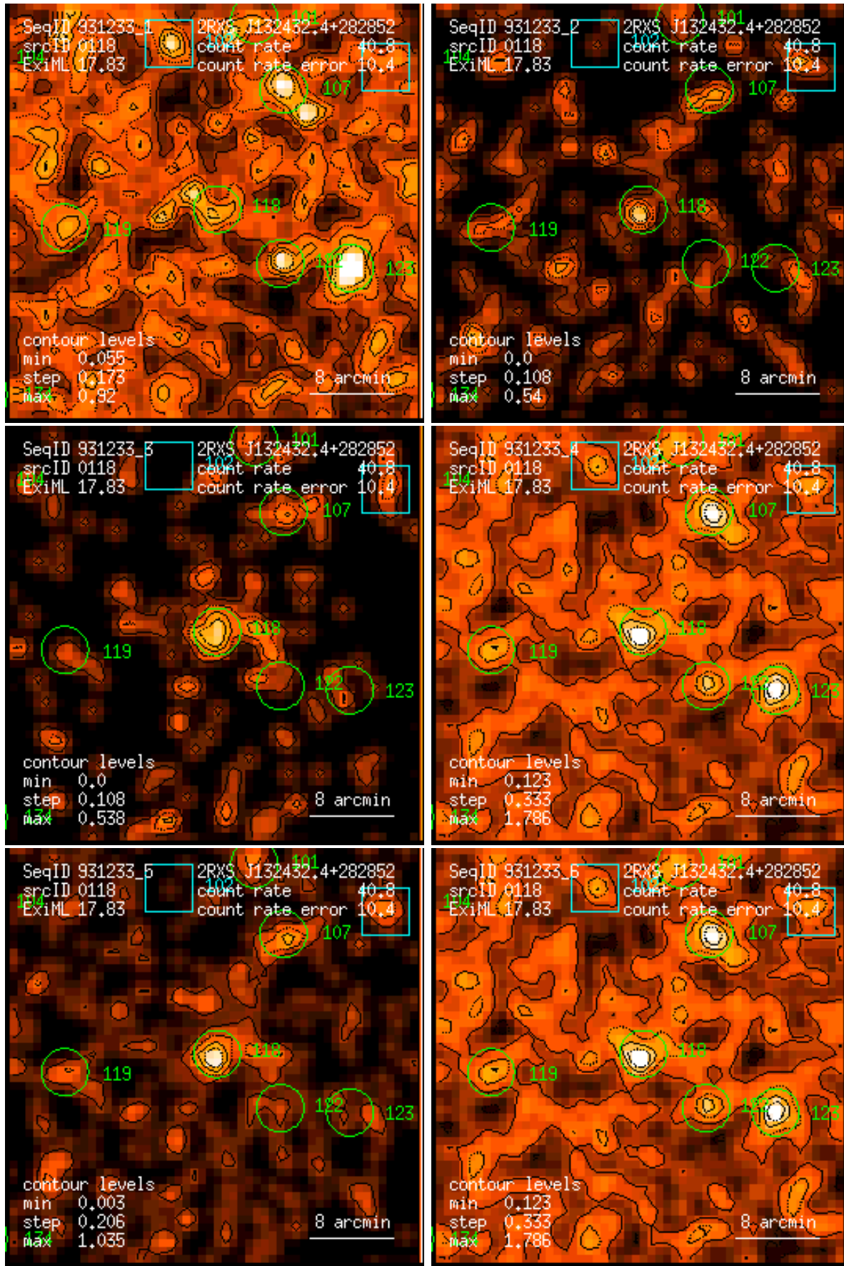
Figure 118: RASS 931233: detection 0118: band rate images, Gaussian filter: (1) PSPC channels 11 – 41, (2) 52 – 90, (3) 91 – 201, (4) 11 – 235, (5) 52 – 201, (6) 11 – 201. Broad band rates in counts/ks. Band rate contour levels in counts/ks/arcmin 2 .
