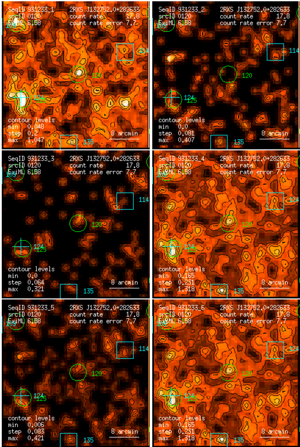
Figure 120: RASS 931233: detection 0120: band rate images, Gaussian filter: (1) PSPC channels 11 – 41, (2) 52 – 90, (3) 91 – 201, (4) 11 – 235, (5) 52 – 201, (6) 11 – 201. Broad band rates in counts/ks. Band rate contour levels in counts/ks/arcmin 2 .
