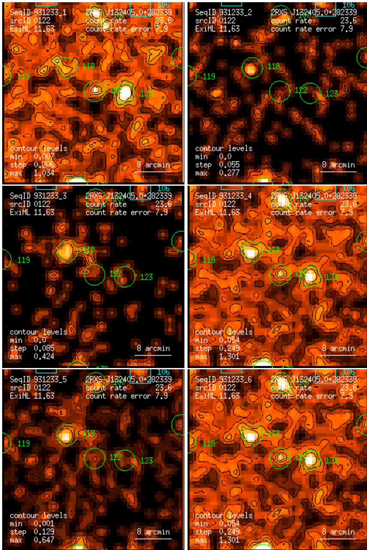
Figure 122: RASS 931233: detection 0122: band rate images, Gaussian filter: (1) PSPC channels 11 – 41, (2) 52 – 90, (3) 91 – 201, (4) 11 – 235, (5) 52 – 201, (6) 11 – 201. Broad band rates in counts/ks. Band rate contour levels in counts/ks/arcmin 2 .
