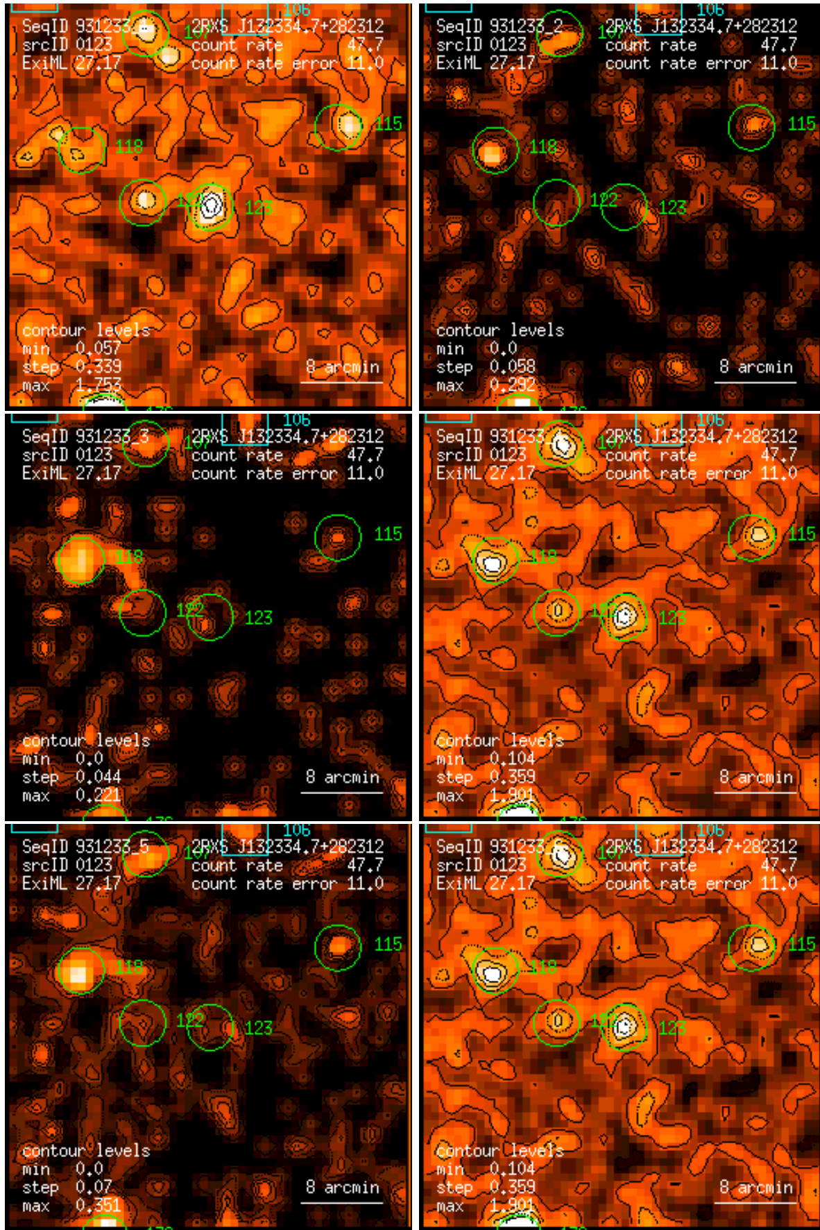
Figure 123: RASS 931233: detection 0123: band rate images, Gaussian filter: (1) PSPC channels 11 – 41, (2) 52 – 90, (3) 91 – 201, (4) 11 – 235, (5) 52 – 201, (6) 11 – 201. Broad band rates in counts/ks. Band rate contour levels in counts/ks/arcmin 2 .
