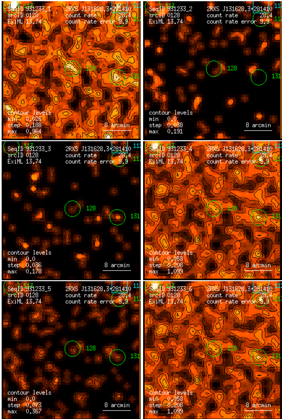
Figure 128: RASS 931233: detection 0128: band rate images, Gaussian filter: (1) PSPC channels 11 – 41, (2) 52 – 90, (3) 91 – 201, (4) 11 – 235, (5) 52 – 201, (6) 11 – 201. Broad band rates in counts/ks. Band rate contour levels in counts/ks/arcmin 2 .
