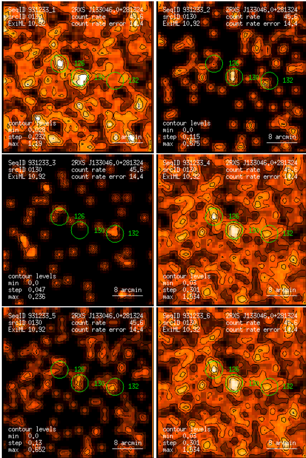
Figure 130: RASS 931233: detection 0130: band rate images, Gaussian filter: (1) PSPC channels 11 – 41, (2) 52 – 90, (3) 91 – 201, (4) 11 – 235, (5) 52 – 201, (6) 11 – 201. Broad band rates in counts/ks. Band rate contour levels in counts/ks/arcmin 2 .
