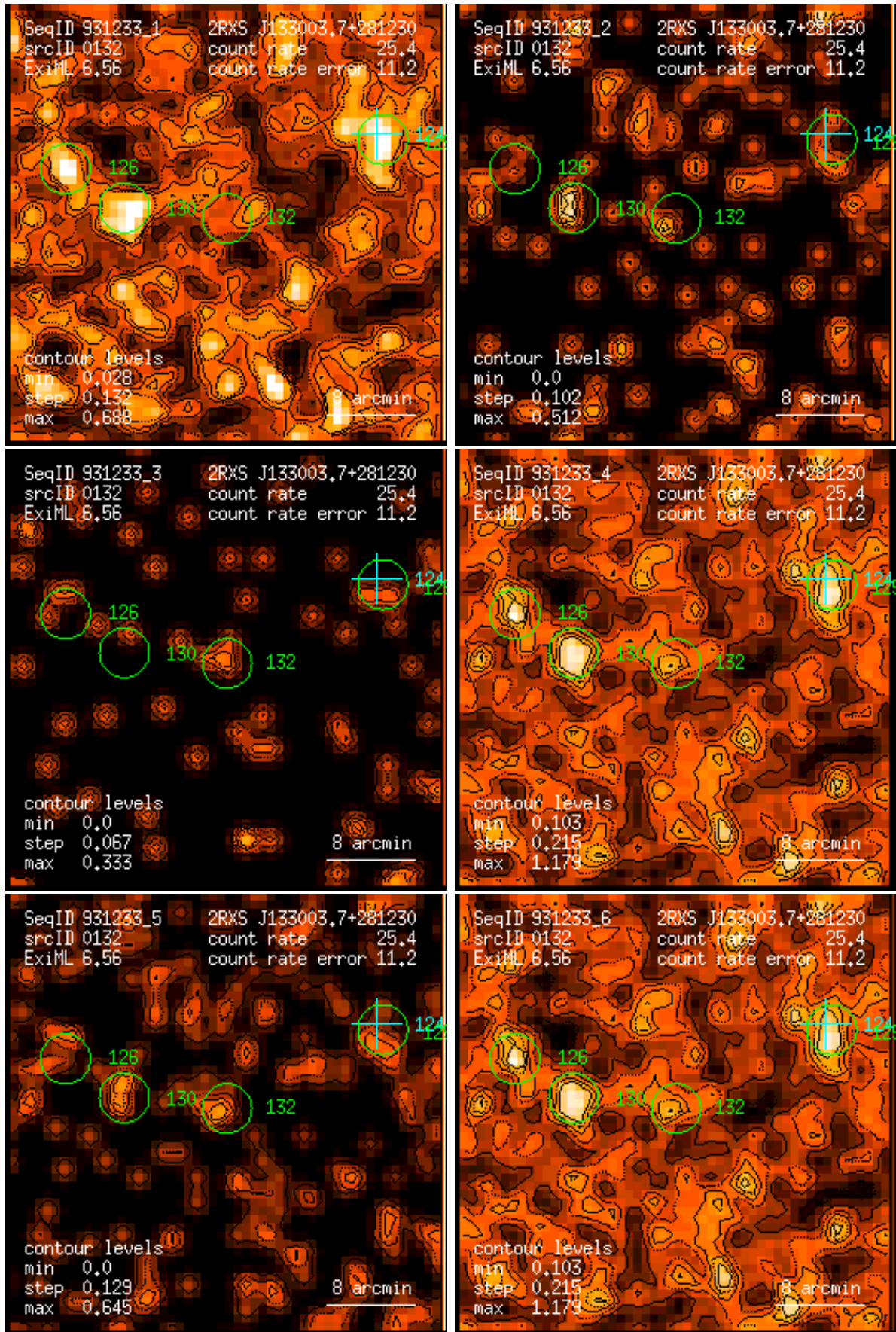
Figure 132: RASS 931233: detection 0132: band rate images, Gaussian filter: (1) PSPC channels 11 – 41, (2) 52 – 90, (3) 91 – 201, (4) 11 – 235, (5) 52 – 201, (6) 11 – 201. Broad band rates in counts/ks. Band rate contour levels in counts/ks/arcmin 2 .
