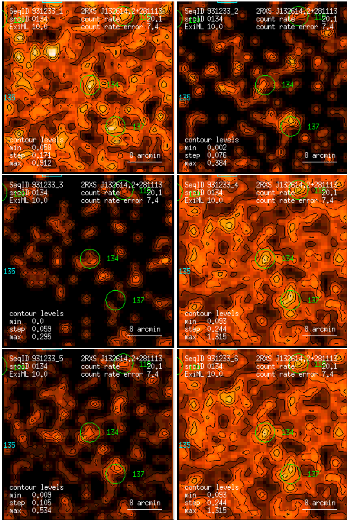
Figure 134: RASS 931233: detection 0134: band rate images, Gaussian filter: (1) PSPC channels 11 – 41, (2) 52 – 90, (3) 91 – 201, (4) 11 – 235, (5) 52 – 201, (6) 11 – 201. Broad band rates in counts/ks. Band rate contour levels in counts/ks/arcmin 2 .
