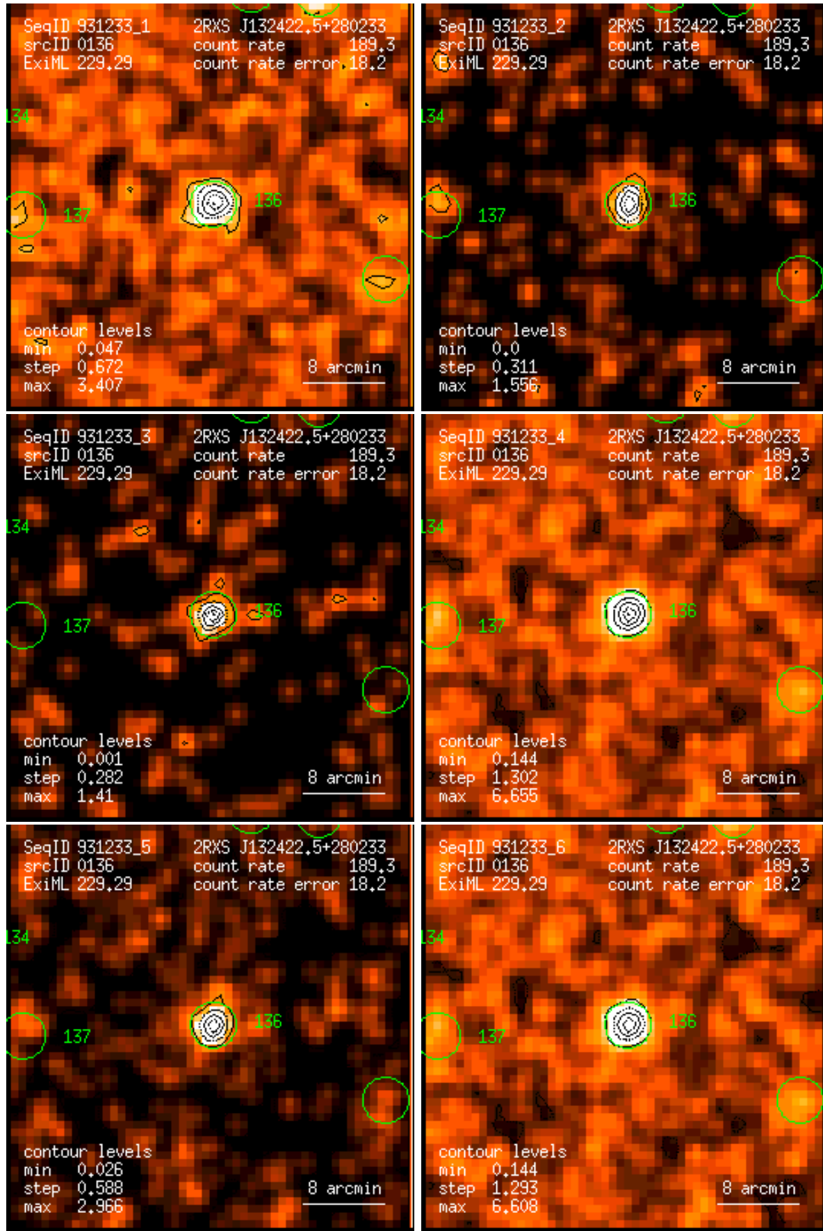
Figure 136: RASS 931233: detection 0136: band rate images, Gaussian filter: (1) PSPC channels 11 – 41, (2) 52 – 90, (3) 91 – 201, (4) 11 – 235, (5) 52 – 201, (6) 11 – 201. Broad band rates in counts/ks. Band rate contour levels in counts/ks/arcmin 2 .
