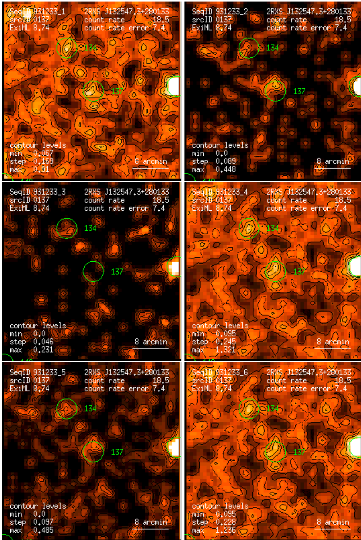
Figure 137: RASS 931233: detection 0137: band rate images, Gaussian filter: (1) PSPC channels 11 – 41, (2) 52 – 90, (3) 91 – 201, (4) 11 – 235, (5) 52 – 201, (6) 11 – 201. Broad band rates in counts/ks. Band rate contour levels in counts/ks/arcmin 2 .
