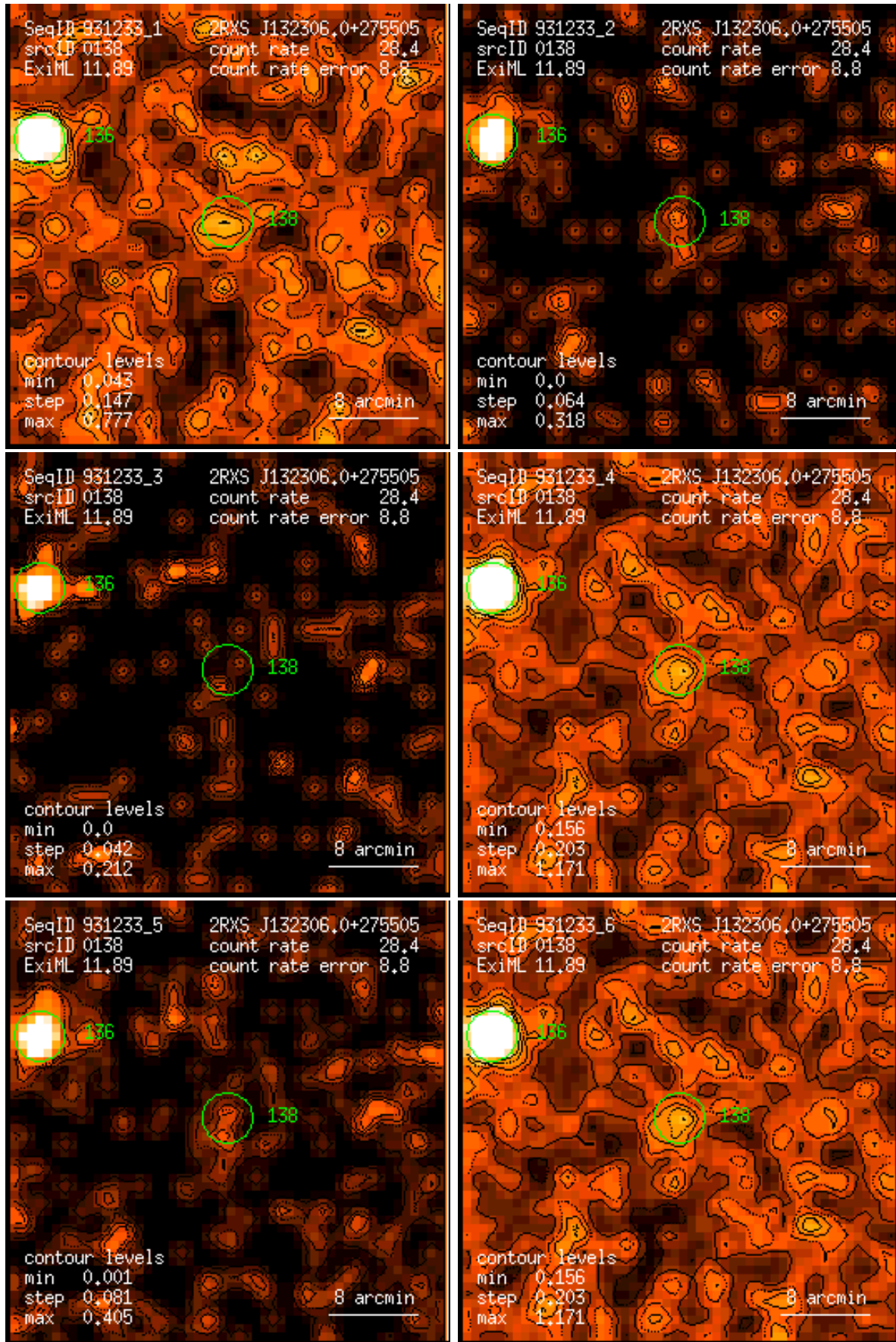
Figure 138: RASS 931233: detection 0138: band rate images, Gaussian filter: (1) PSPC channels 11 – 41, (2) 52 – 90, (3) 91 – 201, (4) 11 – 235, (5) 52 – 201, (6) 11 – 201. Broad band rates in counts/ks. Band rate contour levels in counts/ks/arcmin 2 .
