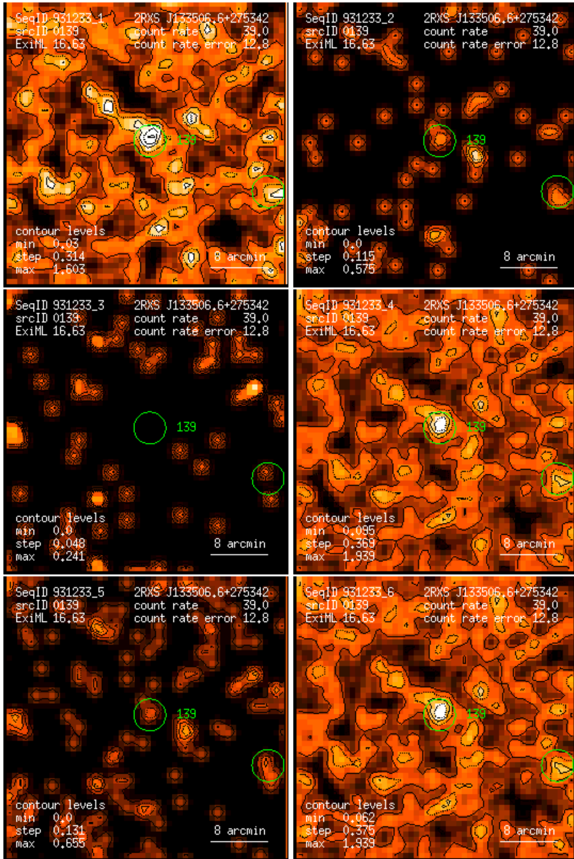
Figure 139: RASS 931233: detection 0139: band rate images, Gaussian filter: (1) PSPC channels 11 – 41, (2) 52 – 90, (3) 91 – 201, (4) 11 – 235, (5) 52 – 201, (6) 11 – 201. Broad band rates in counts/ks. Band rate contour levels in counts/ks/arcmin 2 .
