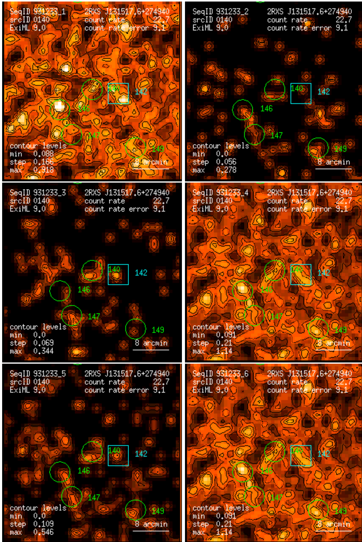
Figure 140: RASS 931233: detection 0140: band rate images, Gaussian filter: (1) PSPC channels 11 – 41, (2) 52 – 90, (3) 91 – 201, (4) 11 – 235, (5) 52 – 201, (6) 11 – 201. Broad band rates in counts/ks. Band rate contour levels in counts/ks/arcmin 2 .
