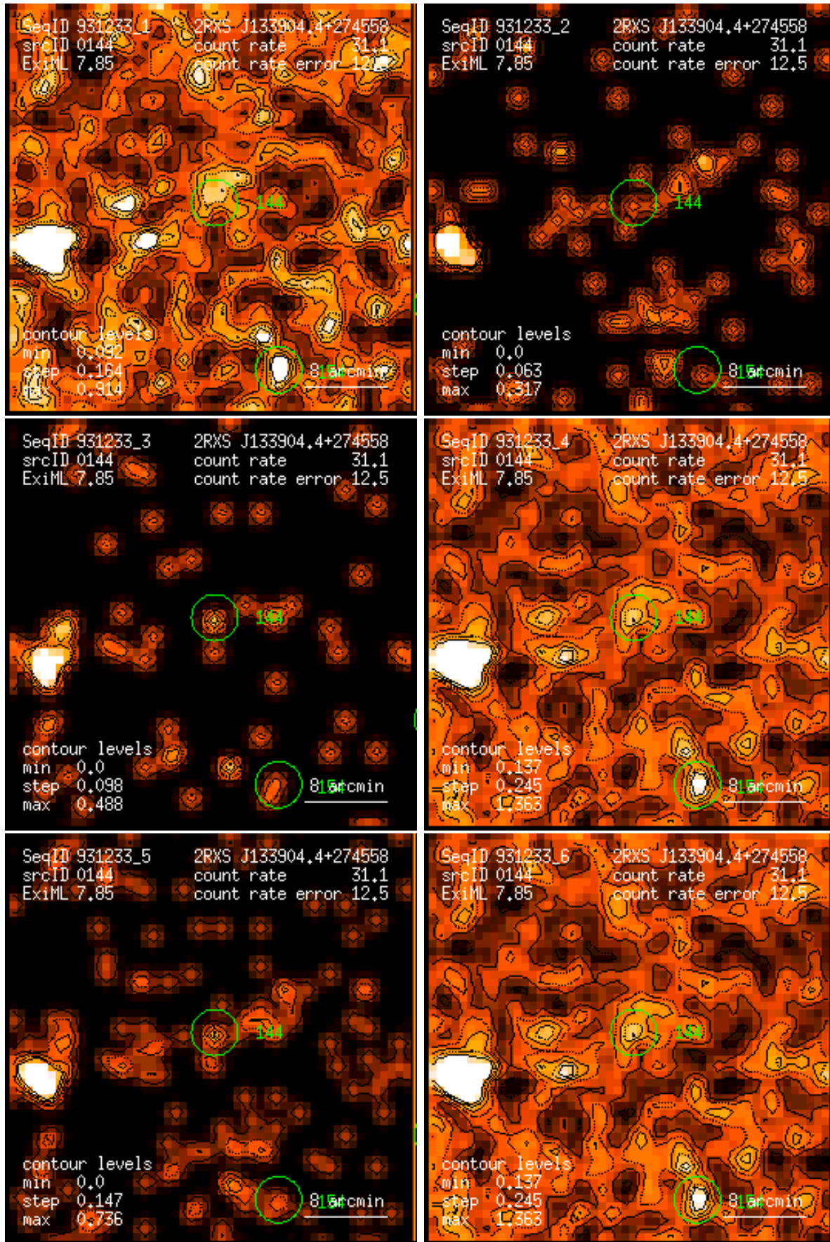
Figure 144: RASS 931233: detection 0144: band rate images, Gaussian filter: (1) PSPC channels 11 – 41, (2) 52 – 90, (3) 91 – 201, (4) 11 – 235, (5) 52 – 201, (6) 11 – 201. Broad band rates in counts/ks. Band rate contour levels in counts/ks/arcmin 2 .
