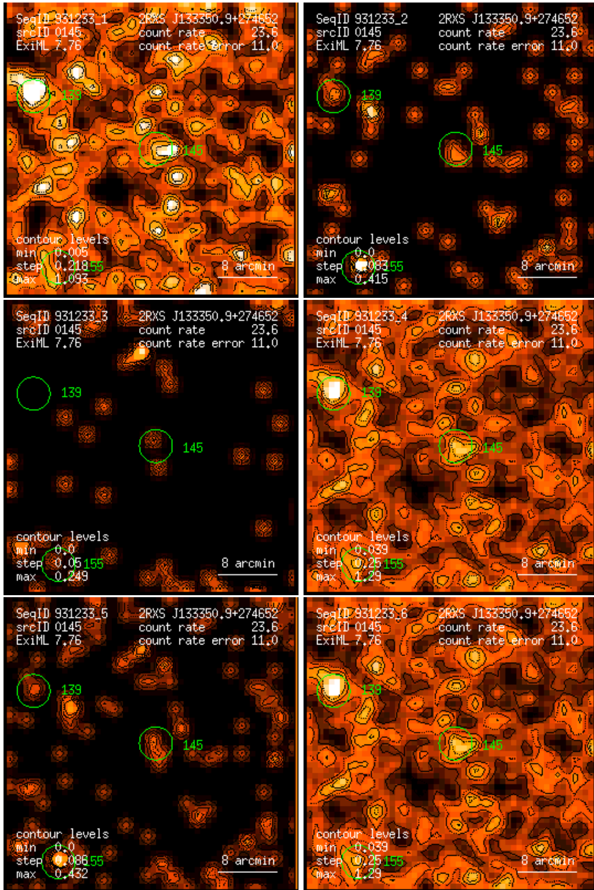
Figure 145: RASS 931233: detection 0145: band rate images, Gaussian filter: (1) PSPC channels 11 – 41, (2) 52 – 90, (3) 91 – 201, (4) 11 – 235, (5) 52 – 201, (6) 11 – 201. Broad band rates in counts/ks. Band rate contour levels in counts/ks/arcmin 2 .
