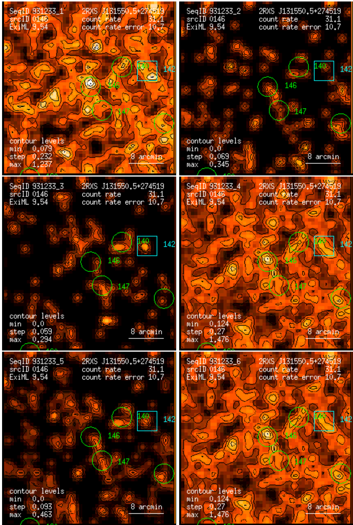
Figure 146: RASS 931233: detection 0146: band rate images, Gaussian filter: (1) PSPC channels 11 – 41, (2) 52 – 90, (3) 91 – 201, (4) 11 – 235, (5) 52 – 201, (6) 11 – 201. Broad band rates in counts/ks. Band rate contour levels in counts/ks/arcmin 2 .
