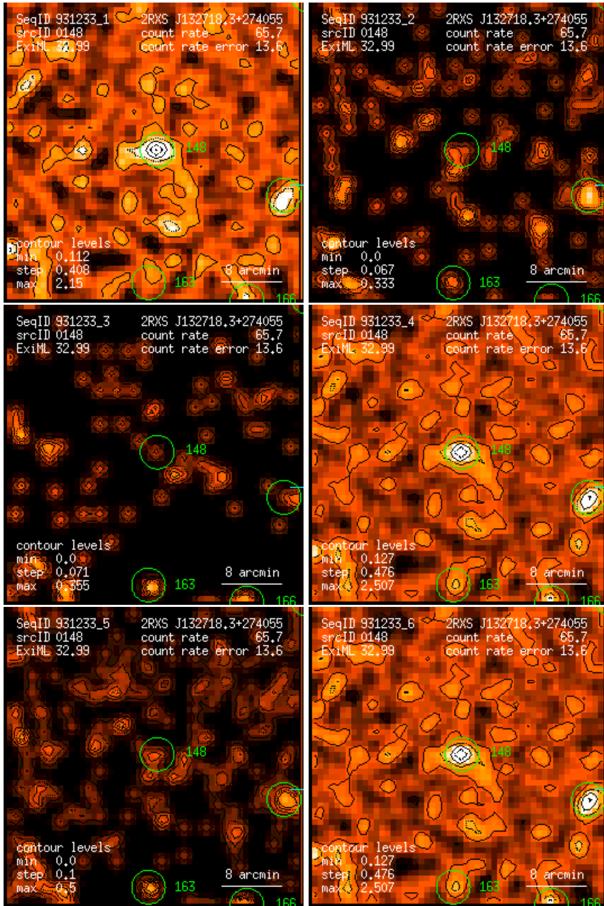
Figure 148: RASS 931233: detection 0148: band rate images, Gaussian filter: (1) PSPC channels 11 – 41, (2) 52 – 90, (3) 91 – 201, (4) 11 – 235, (5) 52 – 201, (6) 11 – 201. Broad band rates in counts/ks. Band rate contour levels in counts/ks/arcmin 2 .
