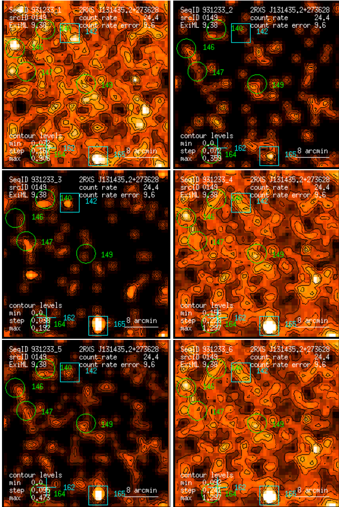
Figure 149: RASS 931233: detection 0149: band rate images, Gaussian filter: (1) PSPC channels 11 – 41, (2) 52 – 90, (3) 91 – 201, (4) 11 – 235, (5) 52 – 201, (6) 11 – 201. Broad band rates in counts/ks. Band rate contour levels in counts/ks/arcmin 2 .
