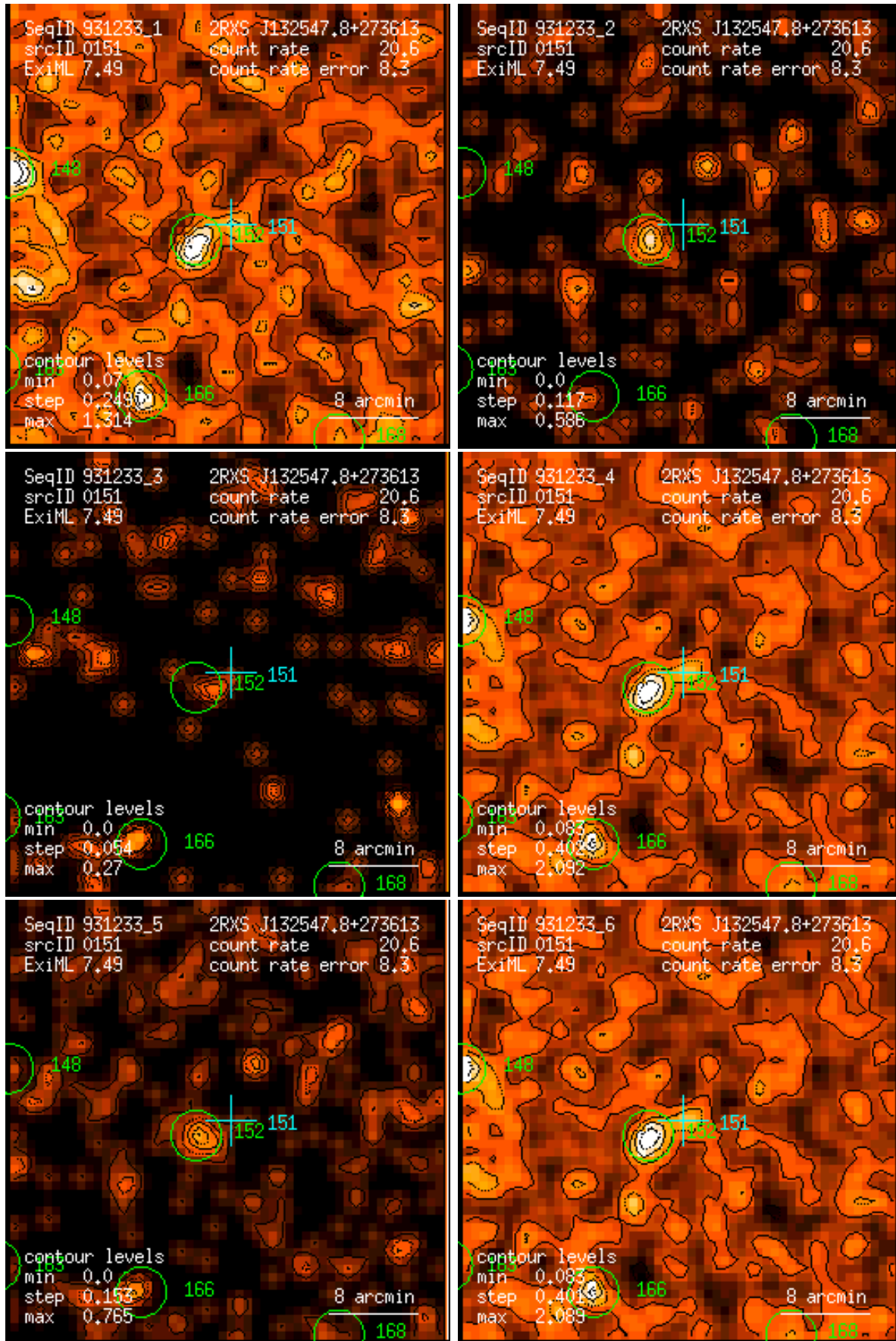
Figure 151: RASS 931233: detection 0151: band rate images, Gaussian filter: (1) PSPC channels 11 – 41, (2) 52 – 90, (3) 91 – 201, (4) 11 – 235, (5) 52 – 201, (6) 11 – 201. Broad band rates in counts/ks. Band rate contour levels in counts/ks/arcmin 2 .
