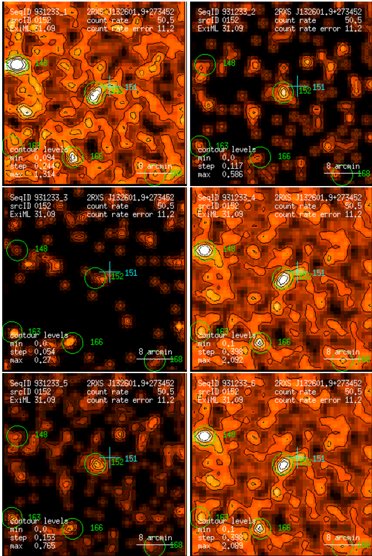
Figure 152: RASS 931233: detection 0152: band rate images, Gaussian filter: (1) PSPC channels 11 – 41, (2) 52 – 90, (3) 91 – 201, (4) 11 – 235, (5) 52 – 201, (6) 11 – 201. Broad band rates in counts/ks. Band rate contour levels in counts/ks/arcmin 2 .
