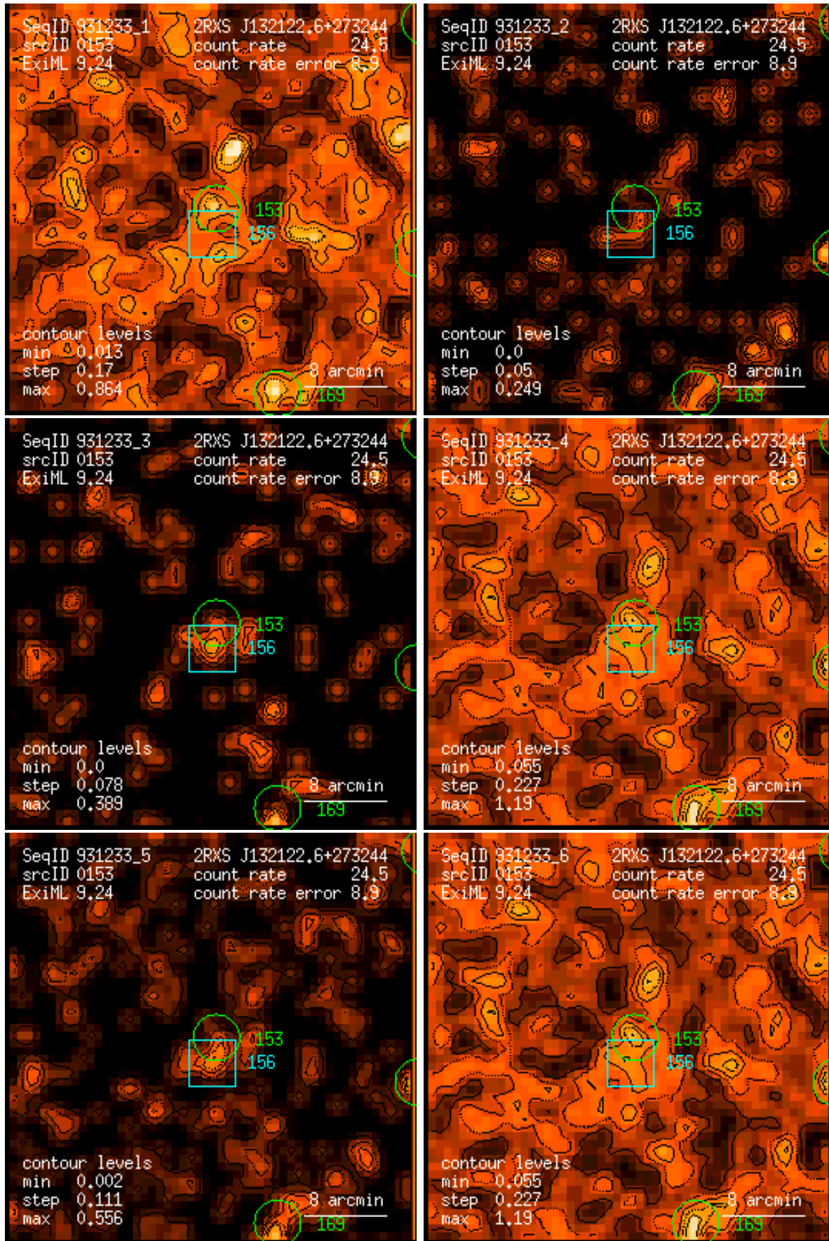
Figure 153: RASS 931233: detection 0153: band rate images, Gaussian filter: (1) PSPC channels 11 – 41, (2) 52 – 90, (3) 91 – 201, (4) 11 – 235, (5) 52 – 201, (6) 11 – 201. Broad band rates in counts/ks. Band rate contour levels in counts/ks/arcmin 2 .
