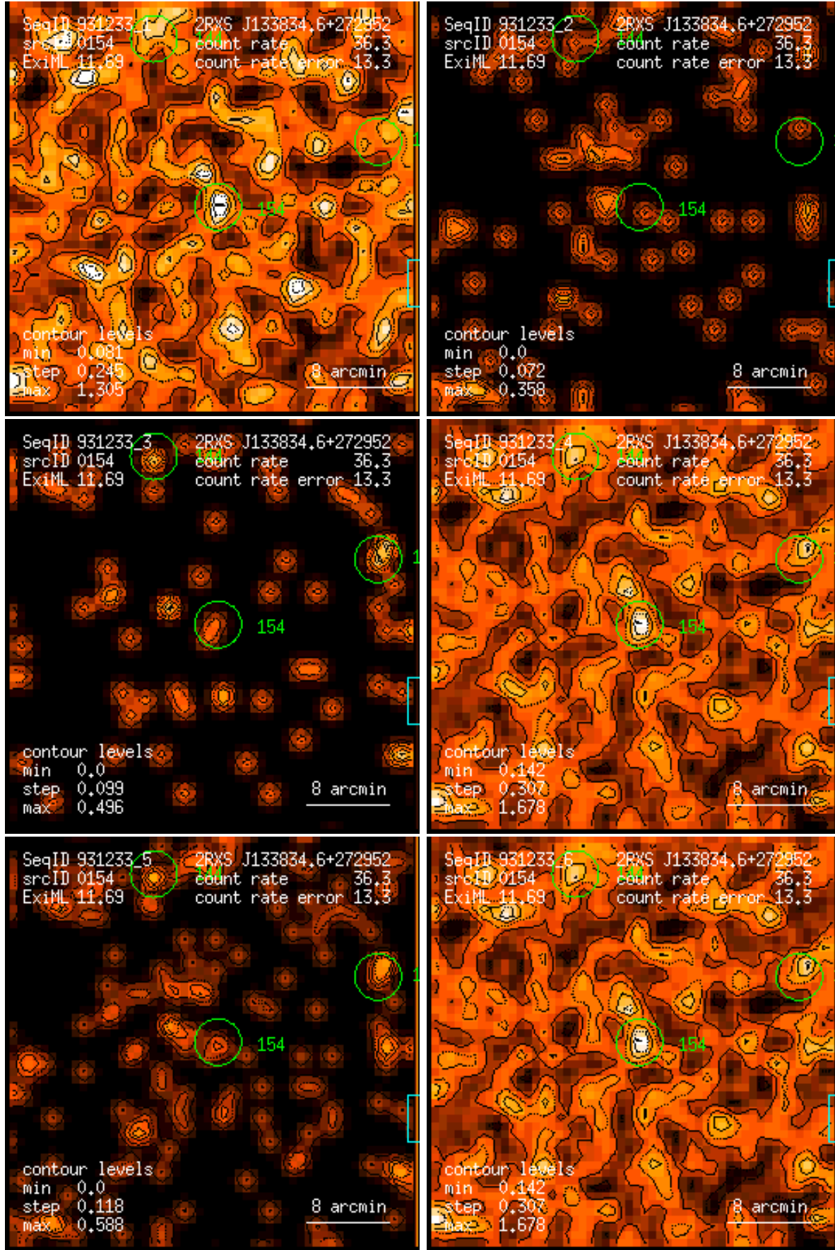
Figure 154: RASS 931233: detection 0154: band rate images, Gaussian filter: (1) PSPC channels 11 – 41, (2) 52 – 90, (3) 91 – 201, (4) 11 – 235, (5) 52 – 201, (6) 11 – 201. Broad band rates in counts/ks. Band rate contour levels in counts/ks/arcmin 2 .
