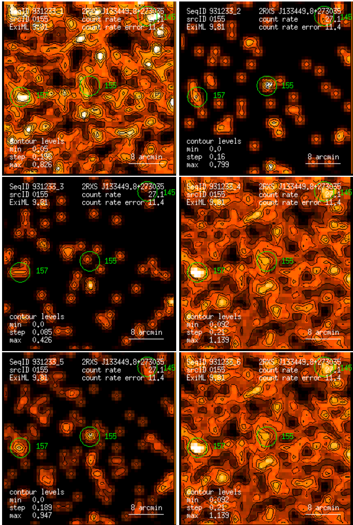
Figure 155: RASS 931233: detection 0155: band rate images, Gaussian filter: (1) PSPC channels 11 – 41, (2) 52 – 90, (3) 91 – 201, (4) 11 – 235, (5) 52 – 201, (6) 11 – 201. Broad band rates in counts/ks. Band rate contour levels in counts/ks/arcmin 2 .
