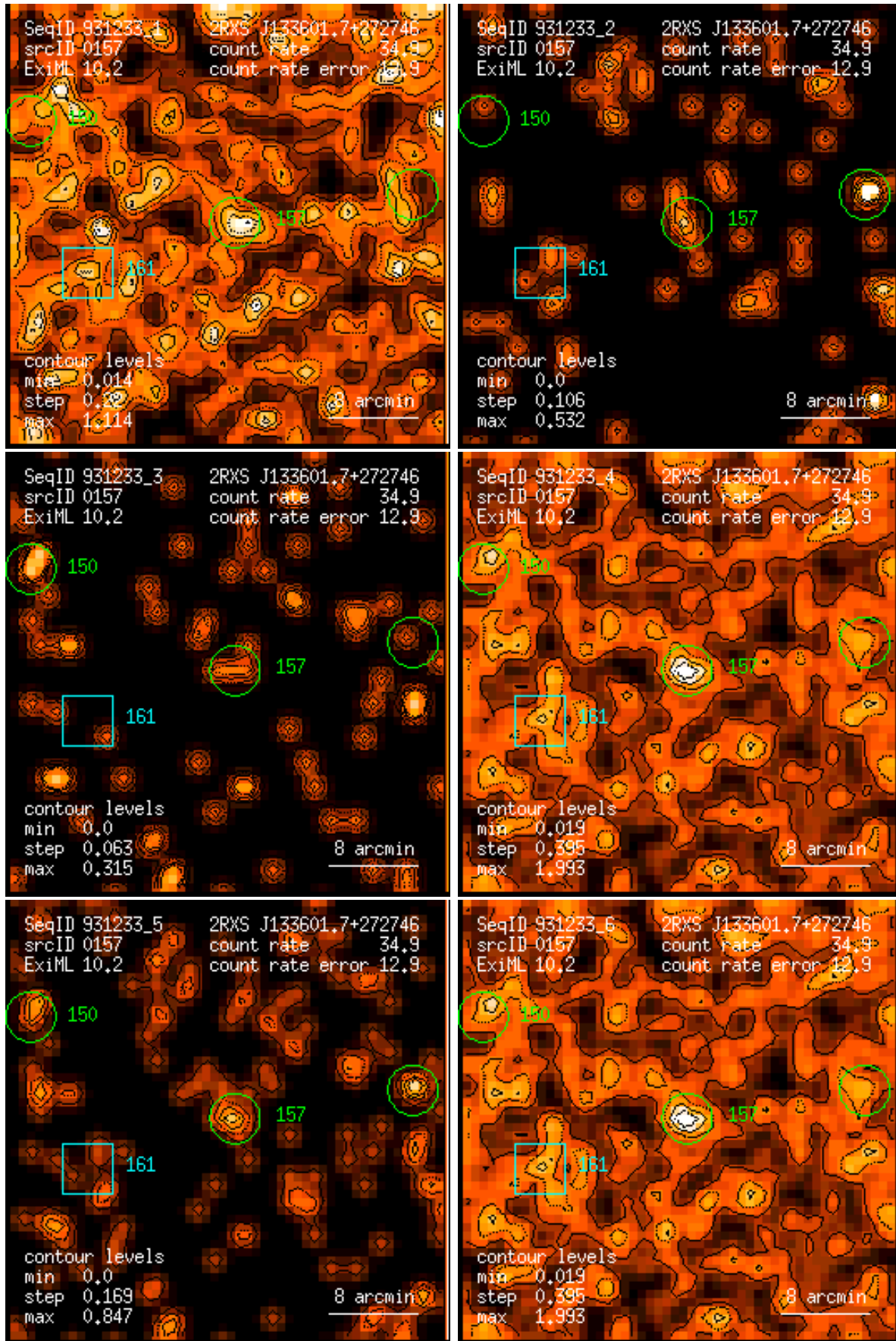
Figure 157: RASS 931233: detection 0157: band rate images, Gaussian filter: (1) PSPC channels 11 – 41, (2) 52 – 90, (3) 91 – 201, (4) 11 – 235, (5) 52 – 201, (6) 11 – 201. Broad band rates in counts/ks. Band rate contour levels in counts/ks/arcmin 2 .
