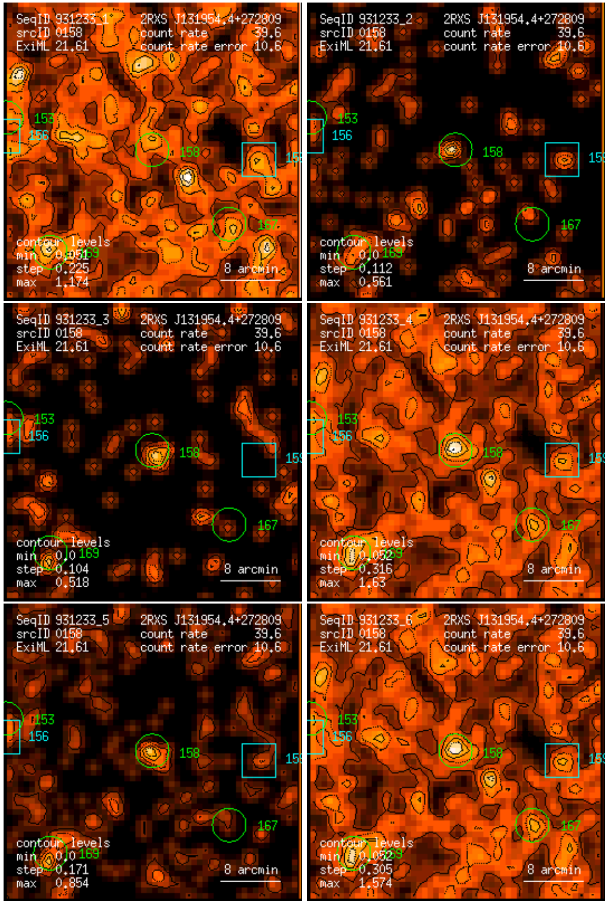
Figure 158: RASS 931233: detection 0158: band rate images, Gaussian filter: (1) PSPC channels 11 – 41, (2) 52 – 90, (3) 91 – 201, (4) 11 – 235, (5) 52 – 201, (6) 11 – 201. Broad band rates in counts/ks. Band rate contour levels in counts/ks/arcmin 2 .
