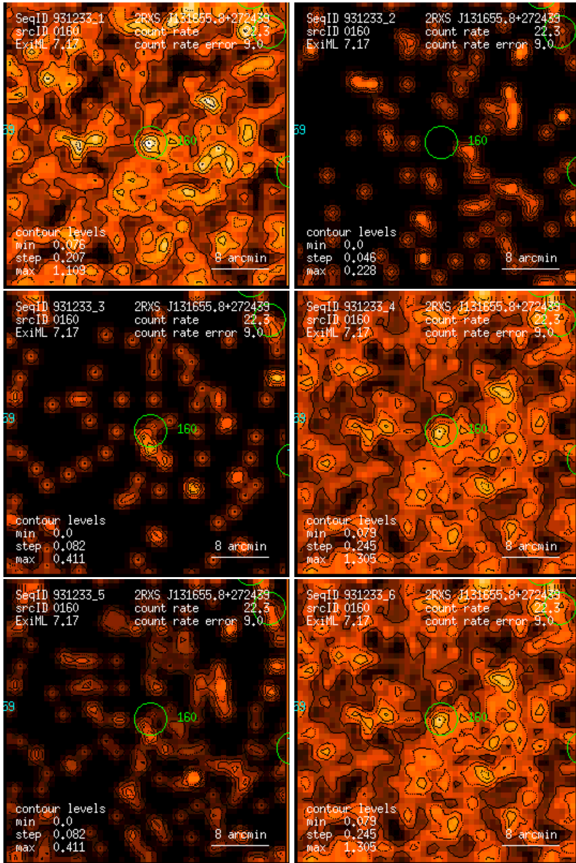
Figure 160: RASS 931233: detection 0160: band rate images, Gaussian filter: (1) PSPC channels 11 – 41, (2) 52 – 90, (3) 91 – 201, (4) 11 – 235, (5) 52 – 201, (6) 11 – 201. Broad band rates in counts/ks. Band rate contour levels in counts/ks/arcmin 2 .
