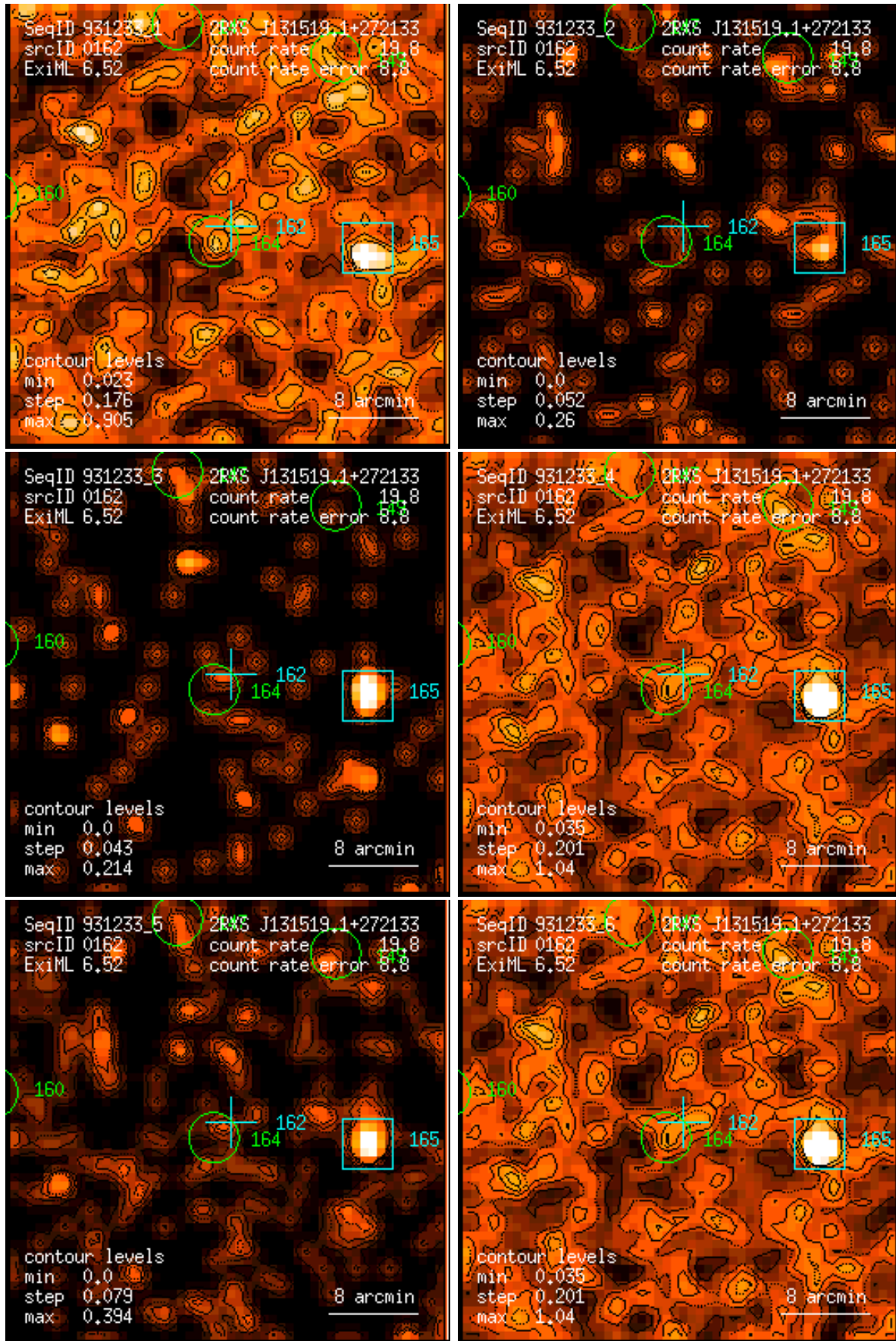
Figure 162: RASS 931233: detection 0162: band rate images, Gaussian filter: (1) PSPC channels 11 – 41, (2) 52 – 90, (3) 91 – 201, (4) 11 – 235, (5) 52 – 201, (6) 11 – 201. Broad band rates in counts/ks. Band rate contour levels in counts/ks/arcmin 2 .
