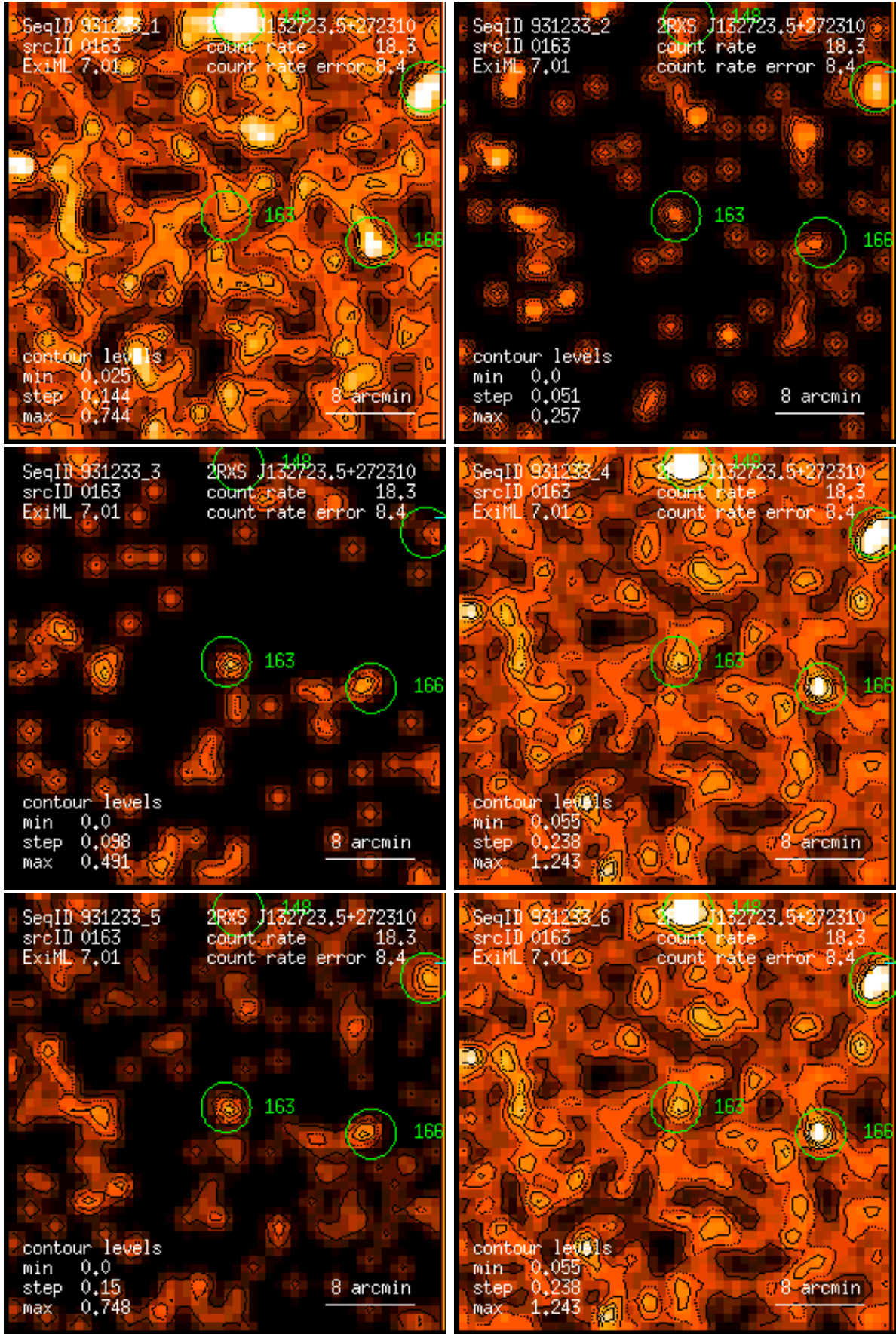
Figure 163: RASS 931233: detection 0163: band rate images, Gaussian filter: (1) PSPC channels 11 – 41, (2) 52 – 90, (3) 91 – 201, (4) 11 – 235, (5) 52 – 201, (6) 11 – 201. Broad band rates in counts/ks. Band rate contour levels in counts/ks/arcmin 2 .
