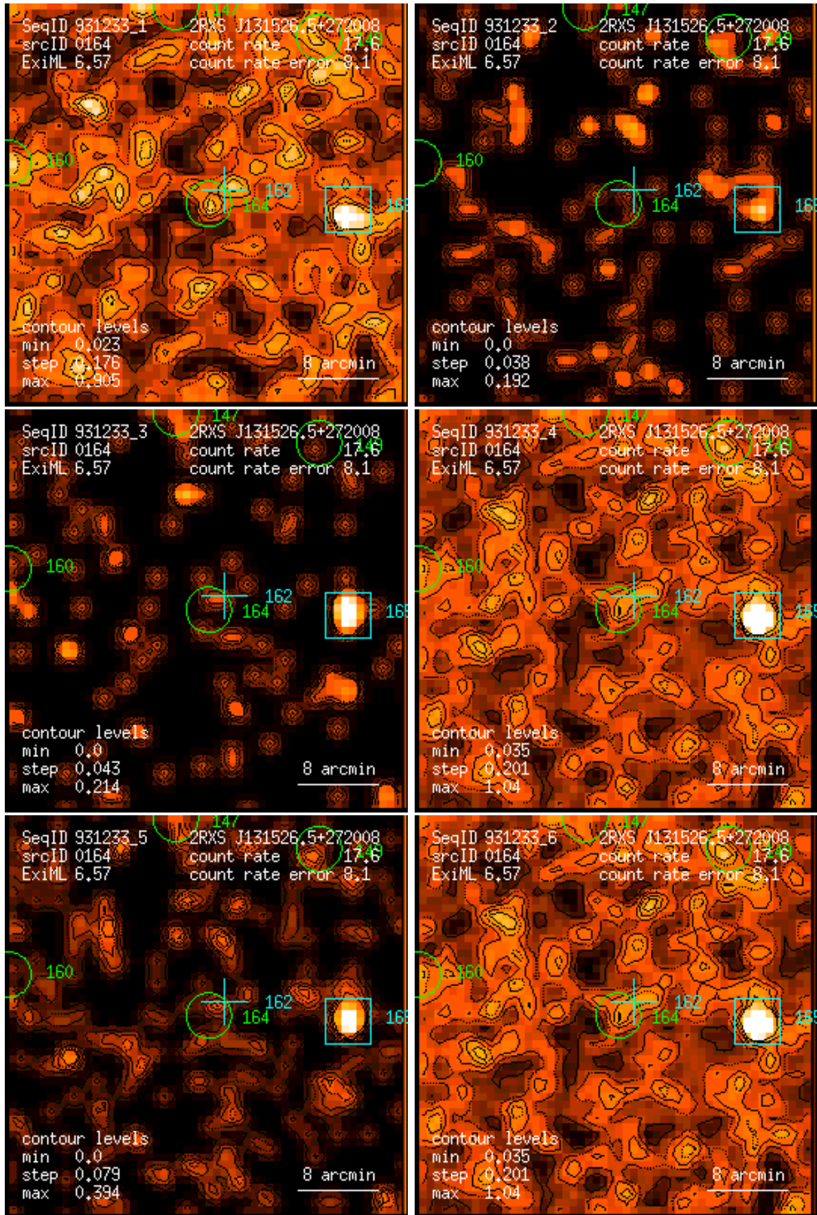
Figure 164: RASS 931233: detection 0164: band rate images, Gaussian filter: (1) PSPC channels 11 – 41, (2) 52 – 90, (3) 91 – 201, (4) 11 – 235, (5) 52 – 201, (6) 11 – 201. Broad band rates in counts/ks. Band rate contour levels in counts/ks/arcmin 2 .
