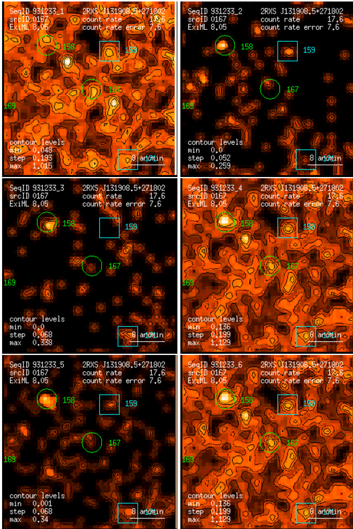
Figure 167: RASS 931233: detection 0167: band rate images, Gaussian filter: (1) PSPC channels 11 – 41, (2) 52 – 90, (3) 91 – 201, (4) 11 – 235, (5) 52 – 201, (6) 11 – 201. Broad band rates in counts/ks. Band rate contour levels in counts/ks/arcmin 2 .
